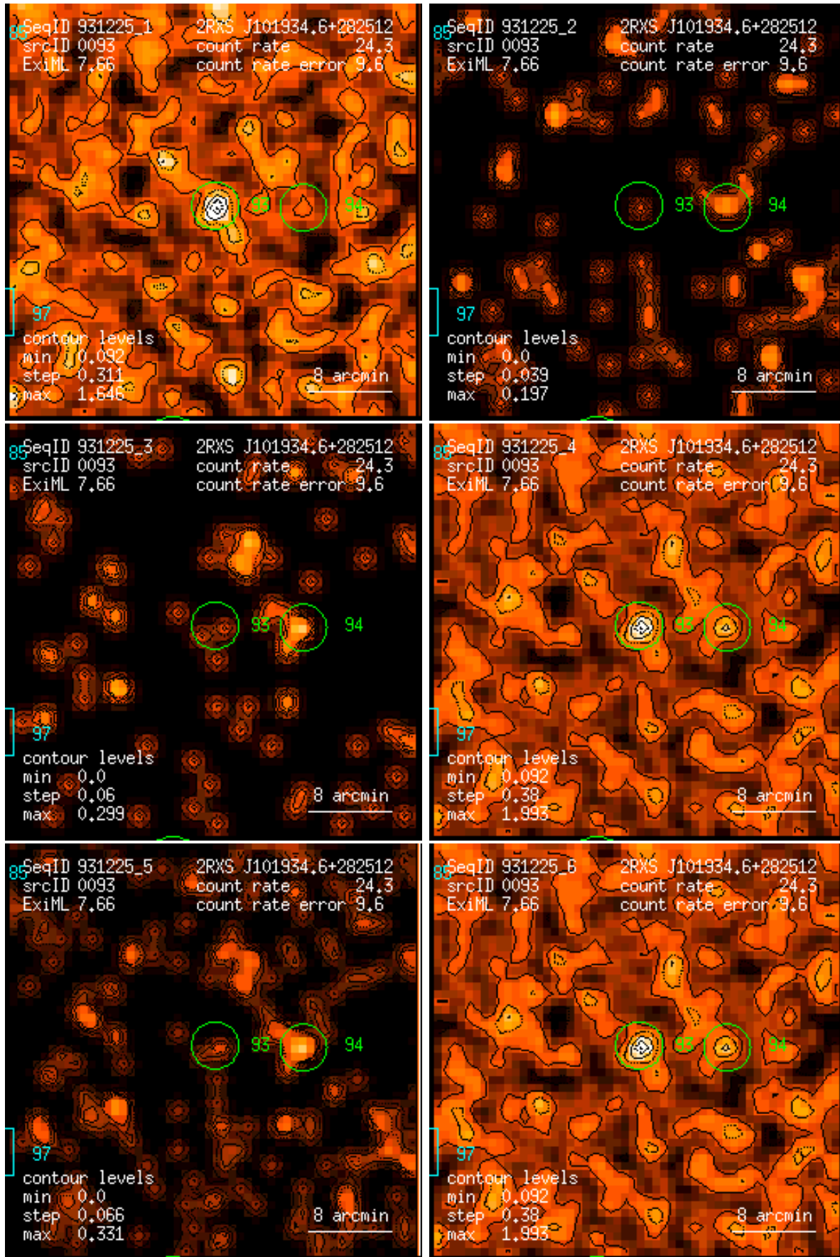
Figure 93: RASS 931225: detection 0093: band rate images, Gaussian filter: (1) PSPC channels 11 – 41, (2) 52 – 90, (3) 91 – 201, (4) 11 – 235, (5) 52 – 201, (6) 11 – 201. Broad band rates in counts/ks. Band rate contour levels in counts/ks/arcmin 2 .
