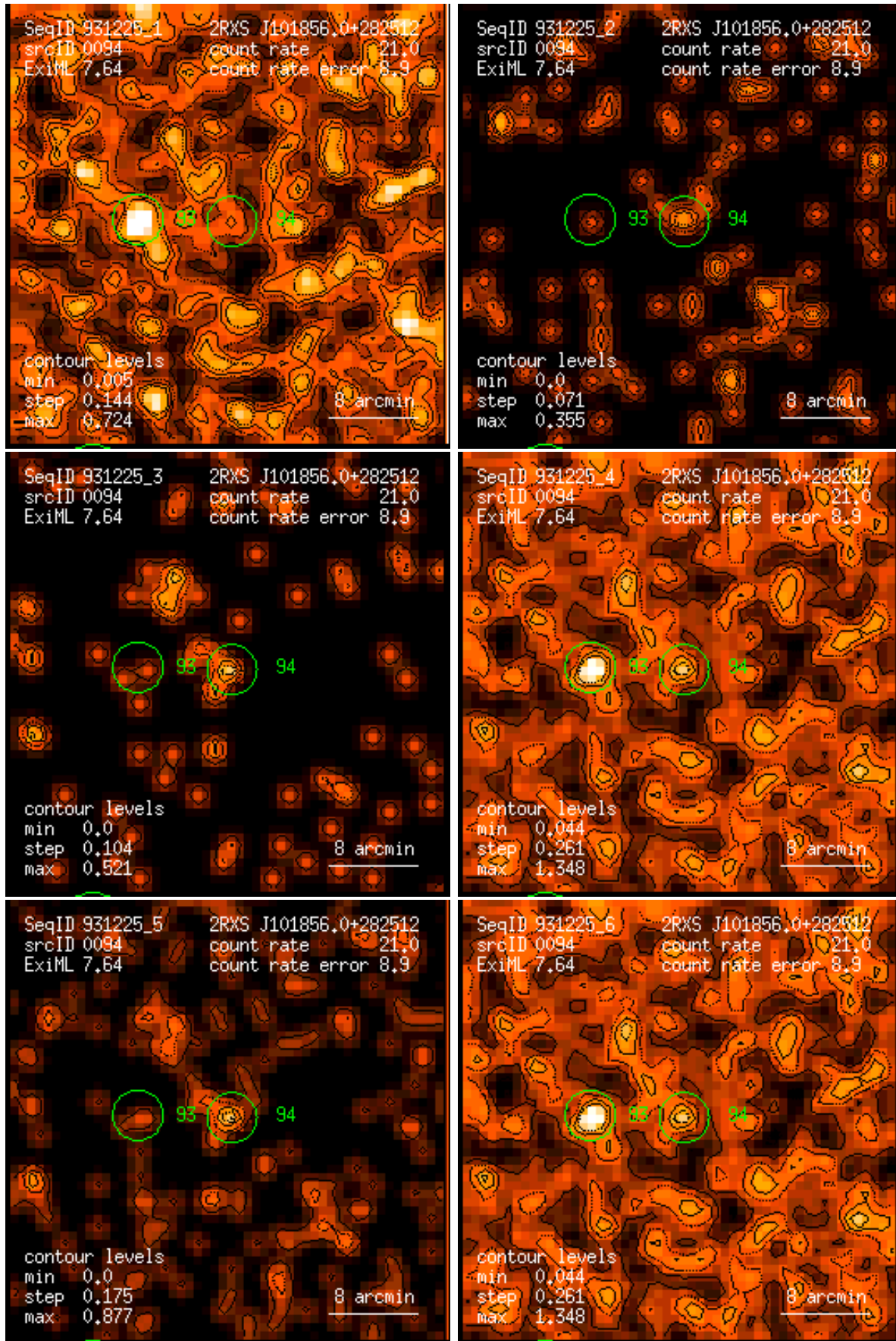
Figure 94: RASS 931225: detection 0094: band rate images, Gaussian filter: (1) PSPC channels 11 – 41, (2) 52 – 90, (3) 91 – 201, (4) 11 – 235, (5) 52 – 201, (6) 11 – 201. Broad band rates in counts/ks. Band rate contour levels in counts/ks/arcmin 2 .
