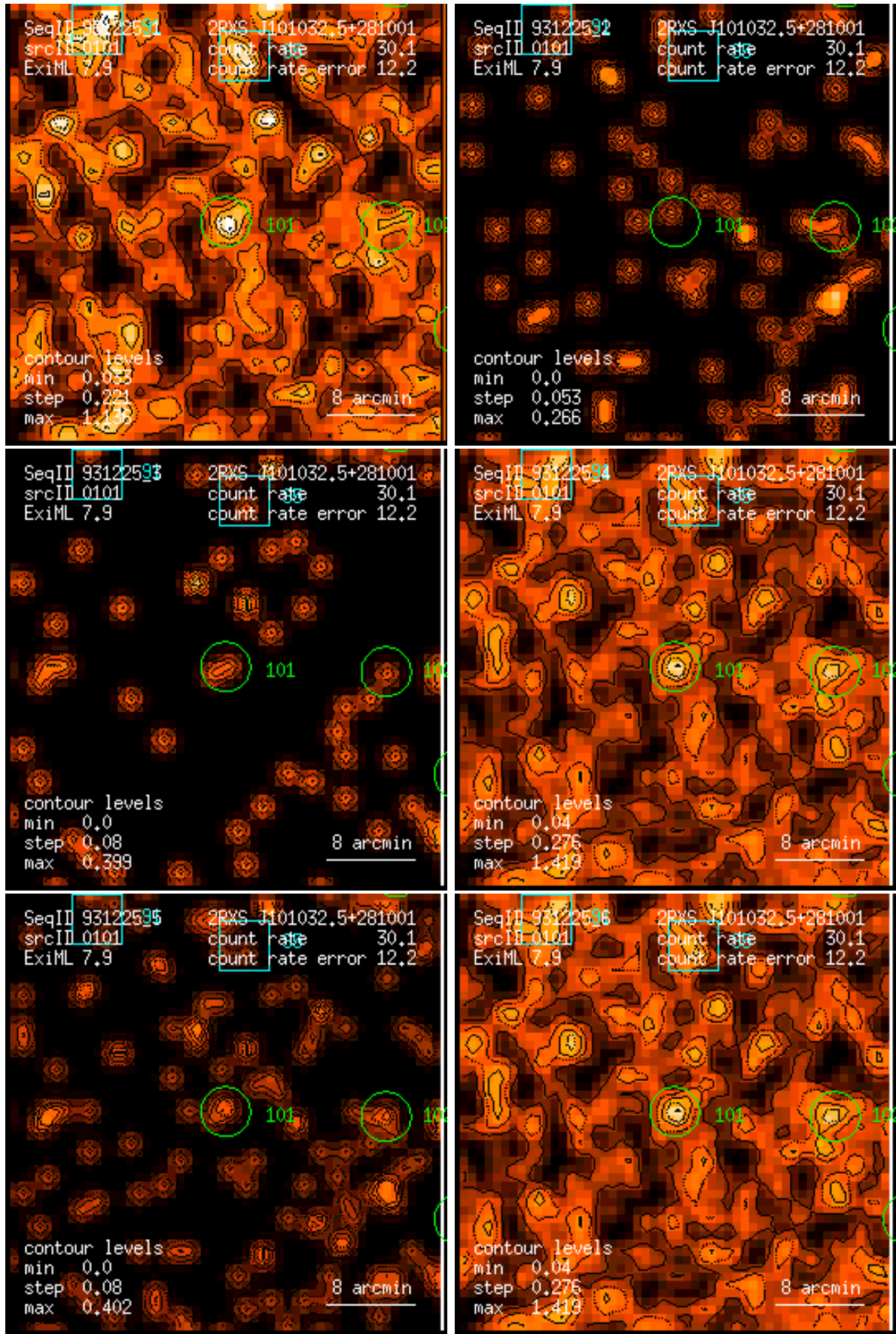
Figure 101: RASS 931225: detection 0101: band rate images, Gaussian filter: (1) PSPC channels 11 – 41, (2) 52 – 90, (3) 91 – 201, (4) 11 – 235, (5) 52 – 201, (6) 11 – 201. Broad band rates in counts/ks. Band rate contour levels in counts/ks/arcmin 2 .
