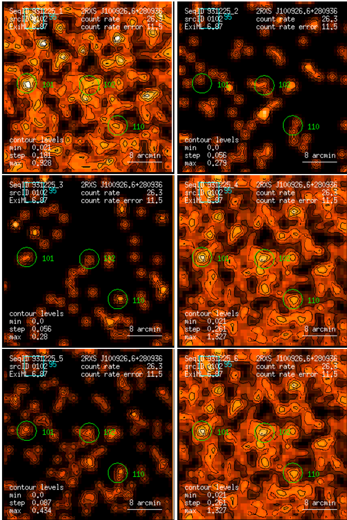
Figure 102: RASS 931225: detection 0102: band rate images, Gaussian filter: (1) PSPC channels 11 – 41, (2) 52 – 90, (3) 91 – 201, (4) 11 – 235, (5) 52 – 201, (6) 11 – 201. Broad band rates in counts/ks. Band rate contour levels in counts/ks/arcmin 2 .
