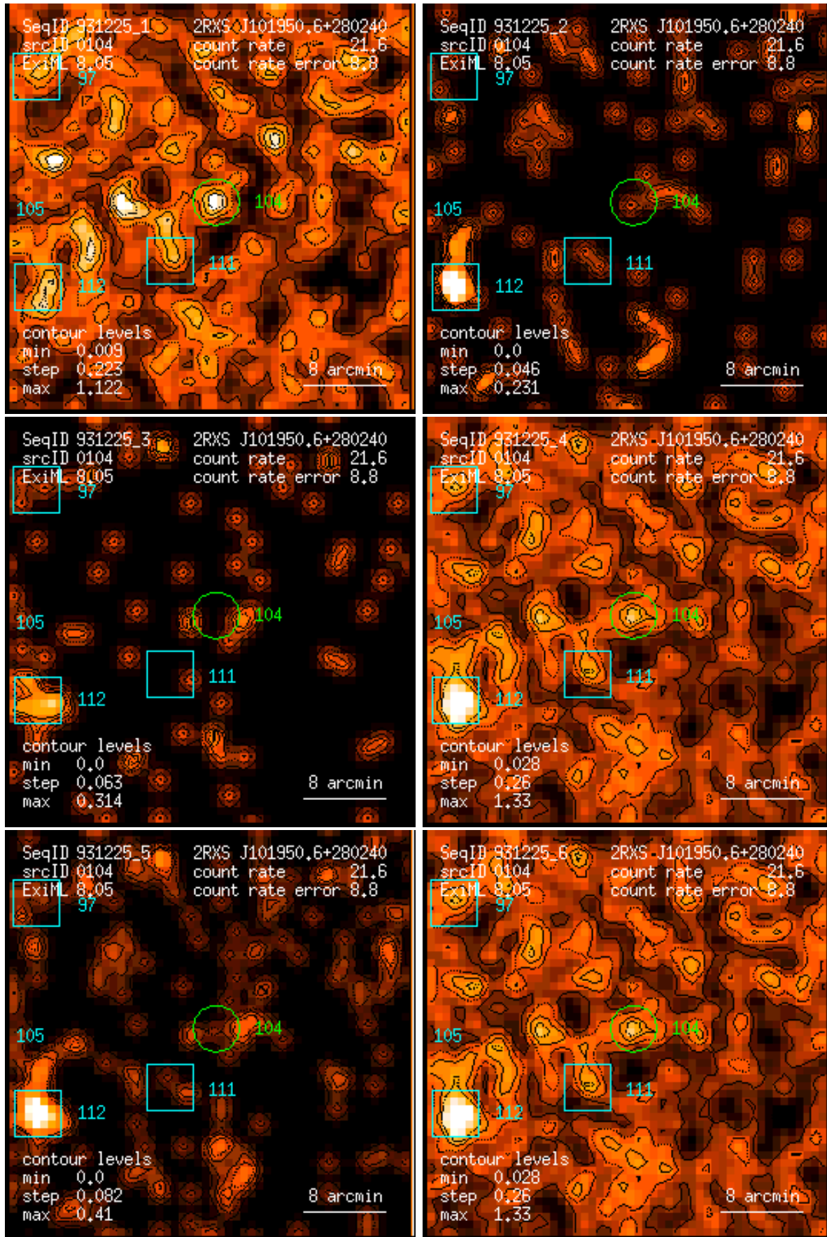
Figure 104: RASS 931225: detection 0104: band rate images, Gaussian filter: (1) PSPC channels 11 – 41, (2) 52 – 90, (3) 91 – 201, (4) 11 – 235, (5) 52 – 201, (6) 11 – 201. Broad band rates in counts/ks. Band rate contour levels in counts/ks/arcmin 2 .
