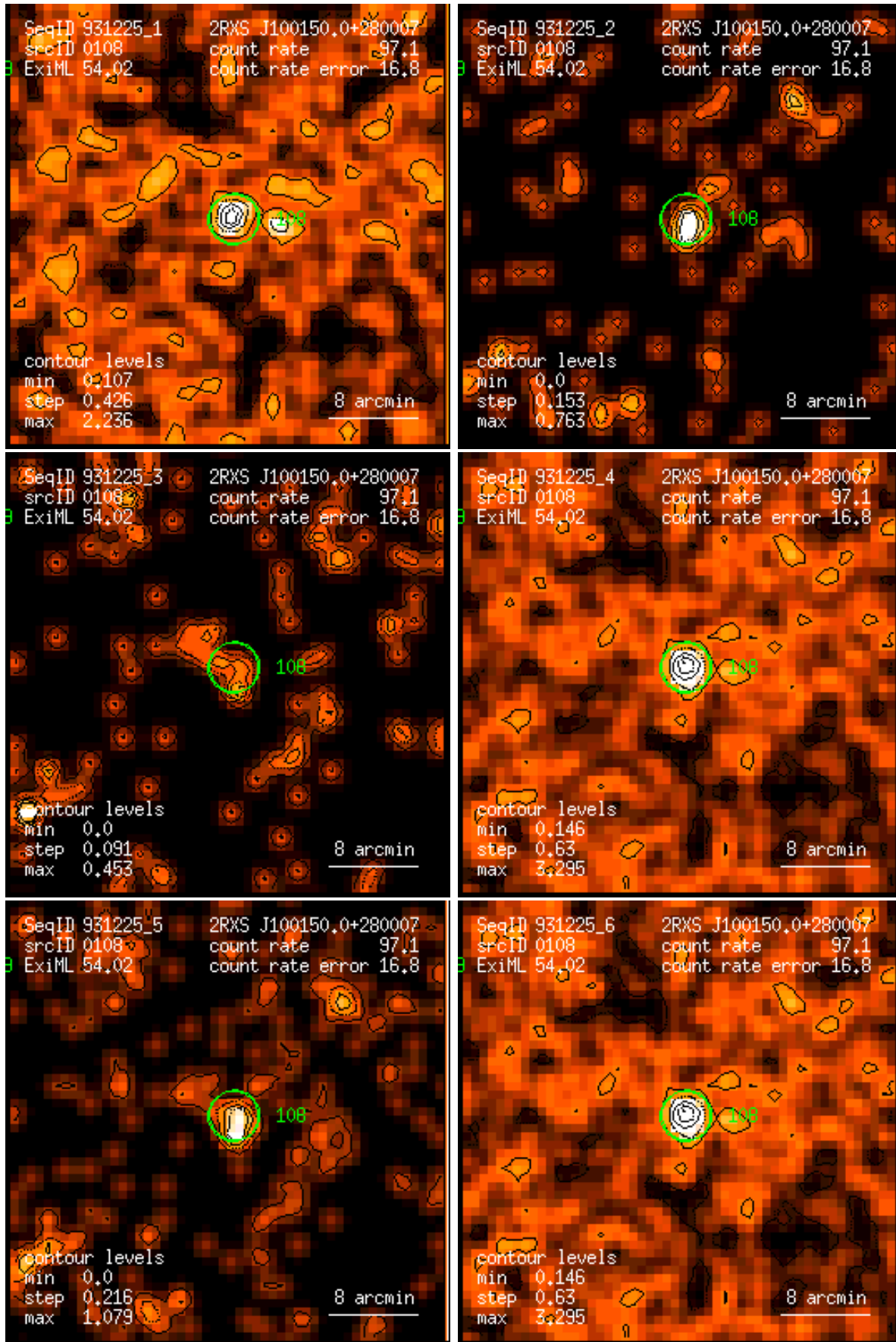
Figure 108: RASS 931225: detection 0108: band rate images, Gaussian filter: (1) PSPC channels 11 – 41, (2) 52 – 90, (3) 91 – 201, (4) 11 – 235, (5) 52 – 201, (6) 11 – 201. Broad band rates in counts/ks. Band rate contour levels in counts/ks/arcmin 2 .
