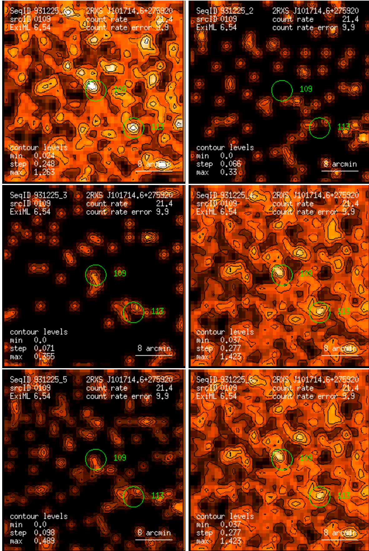
Figure 109: RASS 931225: detection 0109: band rate images, Gaussian filter: (1) PSPC channels 11 – 41, (2) 52 – 90, (3) 91 – 201, (4) 11 – 235, (5) 52 – 201, (6) 11 – 201. Broad band rates in counts/ks. Band rate contour levels in counts/ks/arcmin 2 .
