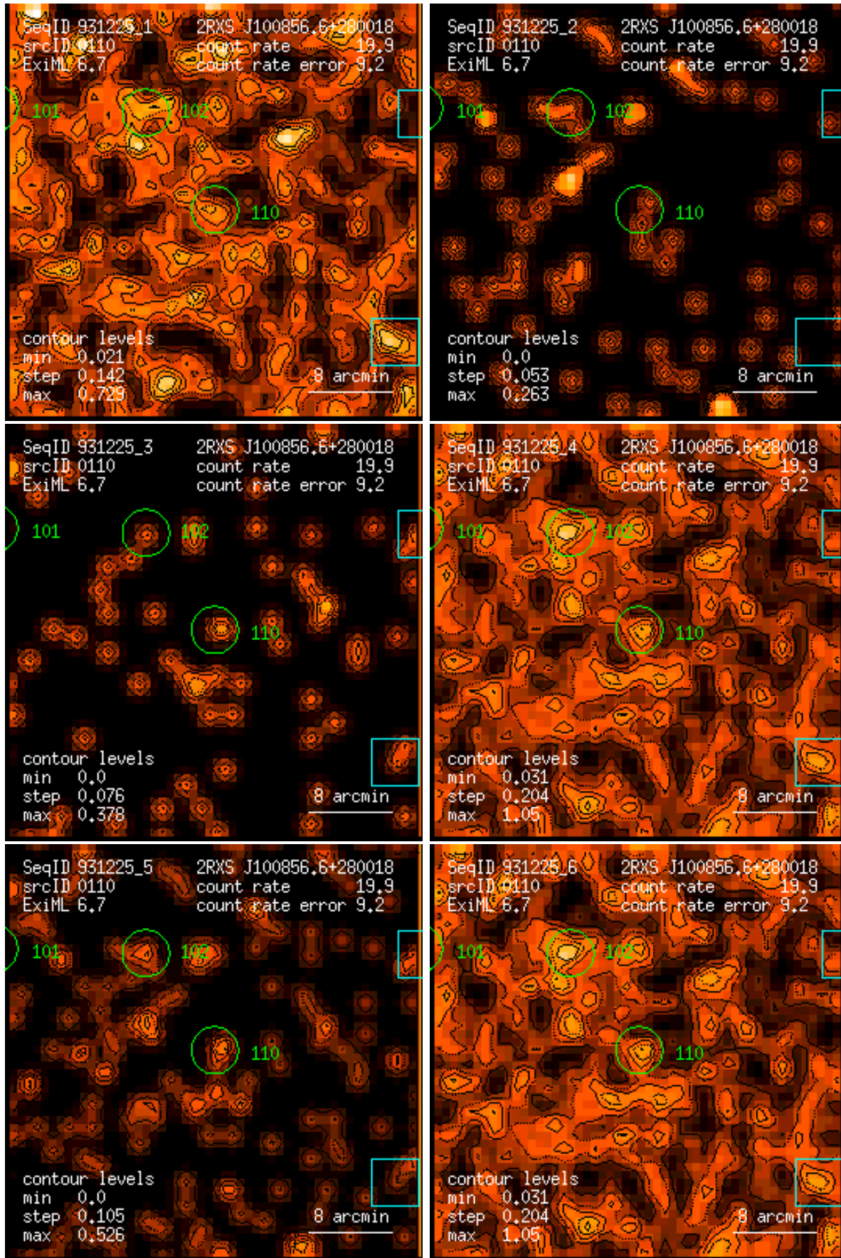
Figure 110: RASS 931225: detection 0110: band rate images, Gaussian filter: (1) PSPC channels 11 – 41, (2) 52 – 90, (3) 91 – 201, (4) 11 – 235, (5) 52 – 201, (6) 11 – 201. Broad band rates in counts/ks. Band rate contour levels in counts/ks/arcmin 2 .
