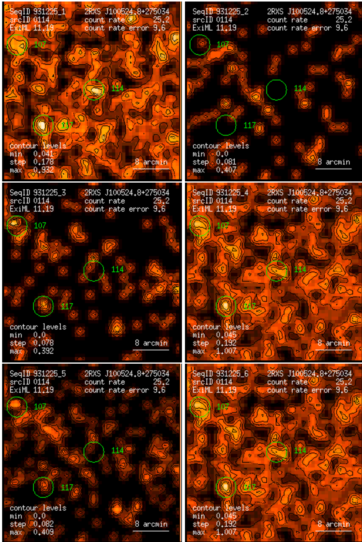
Figure 114: RASS 931225: detection 0114: band rate images, Gaussian filter: (1) PSPC channels 11 – 41, (2) 52 – 90, (3) 91 – 201, (4) 11 – 235, (5) 52 – 201, (6) 11 – 201. Broad band rates in counts/ks. Band rate contour levels in counts/ks/arcmin 2 .
