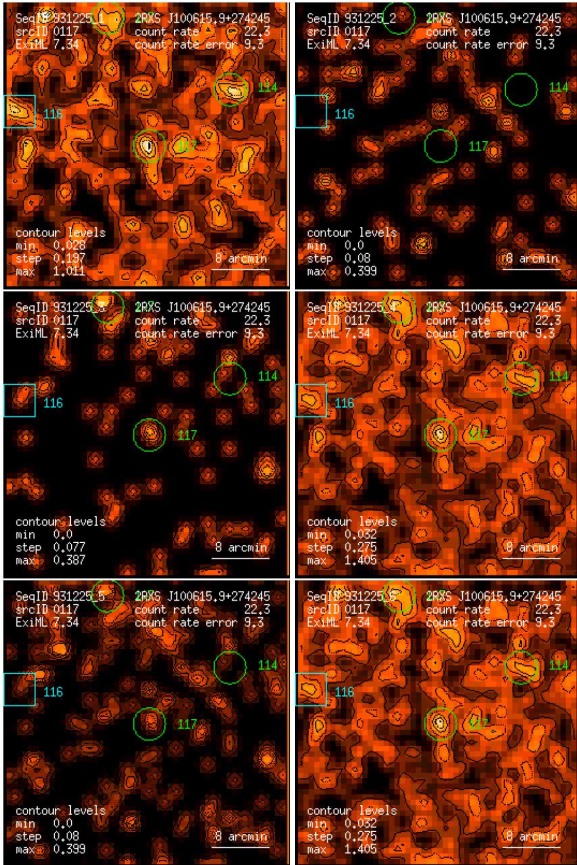
Figure 117: RASS 931225: detection 0117: band rate images, Gaussian filter: (1) PSPC channels 11 – 41, (2) 52 – 90, (3) 91 – 201, (4) 11 – 235, (5) 52 – 201, (6) 11 – 201. Broad band rates in counts/ks. Band rate contour levels in counts/ks/arcmin 2 .
