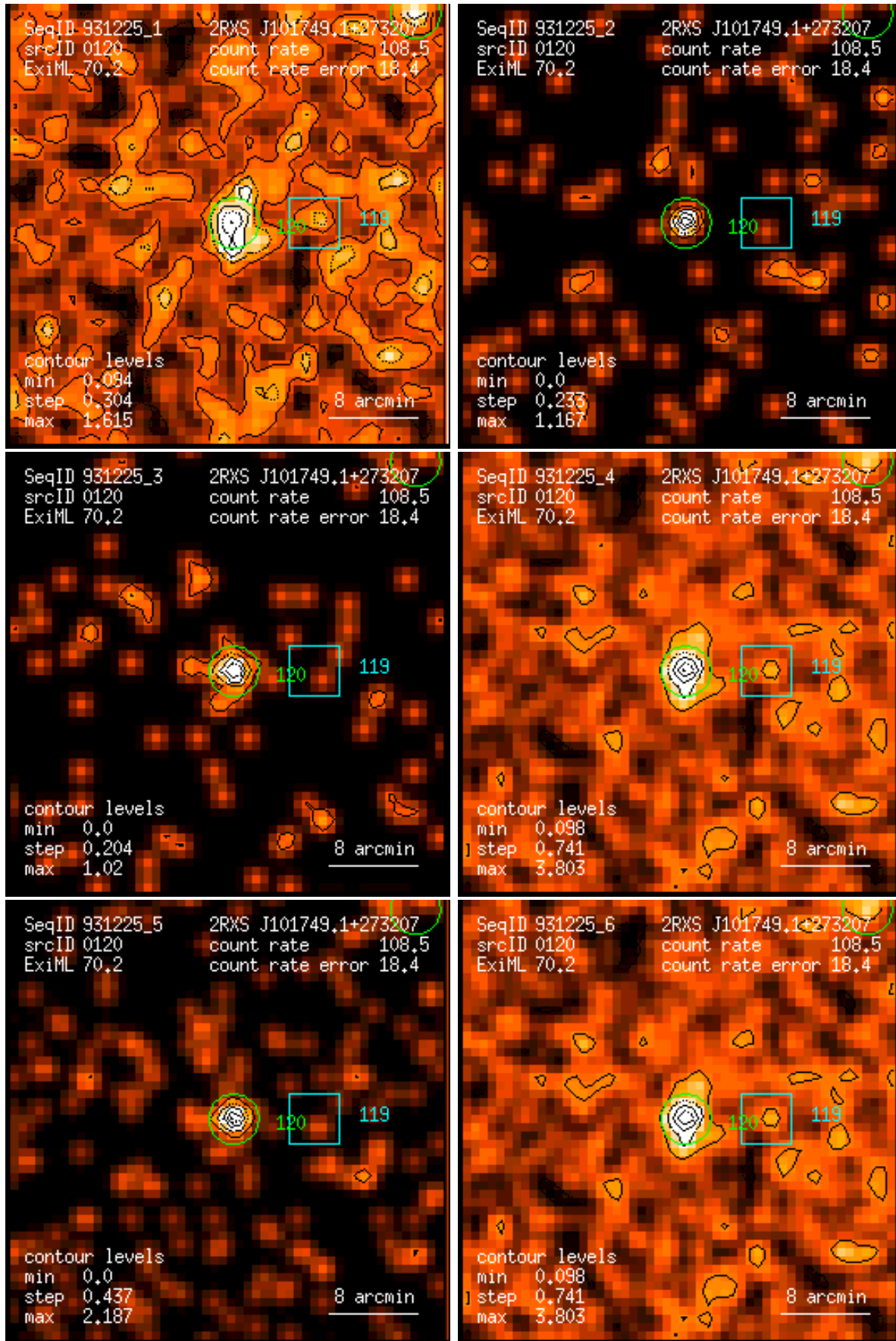
Figure 120: RASS 931225: detection 0120: band rate images, Gaussian filter: (1) PSPC channels 11 – 41, (2) 52 – 90, (3) 91 – 201, (4) 11 – 235, (5) 52 – 201, (6) 11 – 201. Broad band rates in counts/ks. Band rate contour levels in counts/ks/arcmin 2 .
