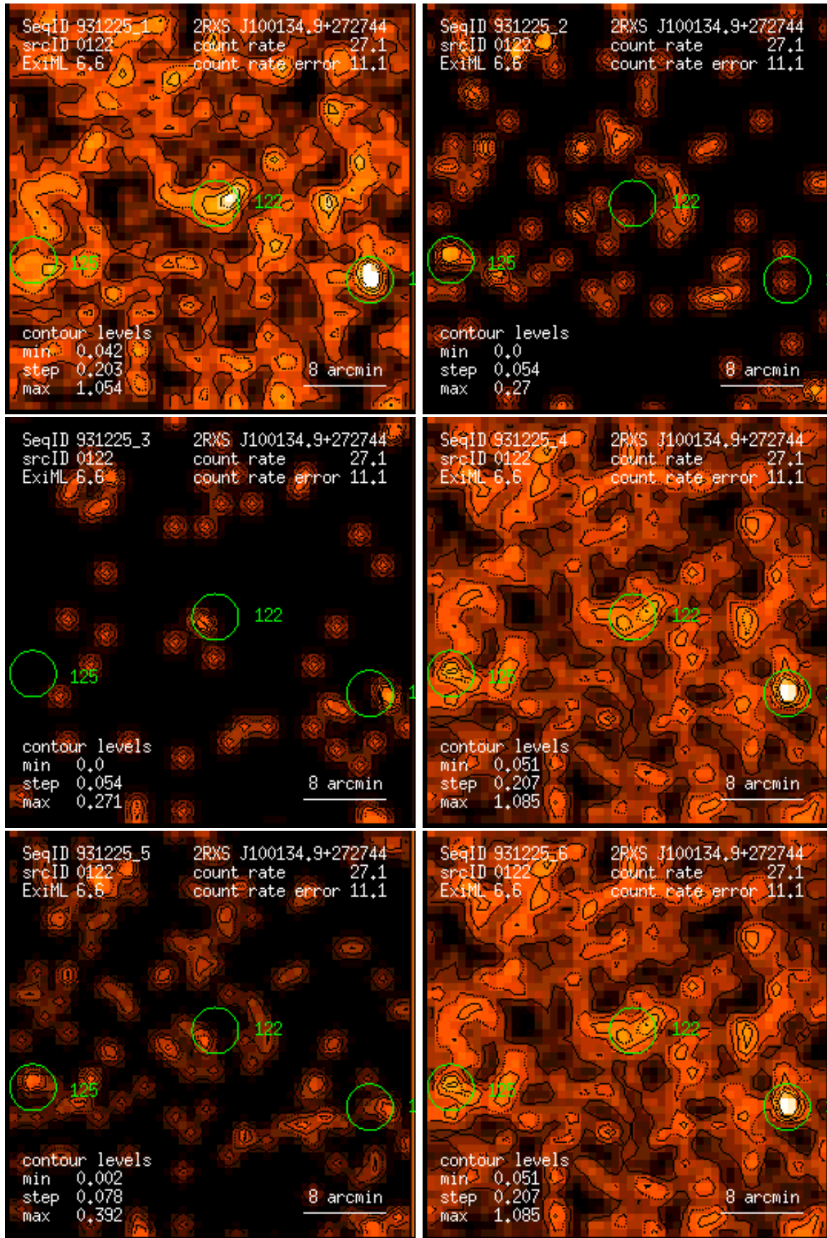
Figure 122: RASS 931225: detection 0122: band rate images, Gaussian filter: (1) PSPC channels 11 – 41, (2) 52 – 90, (3) 91 – 201, (4) 11 – 235, (5) 52 – 201, (6) 11 – 201. Broad band rates in counts/ks. Band rate contour levels in counts/ks/arcmin 2 .
