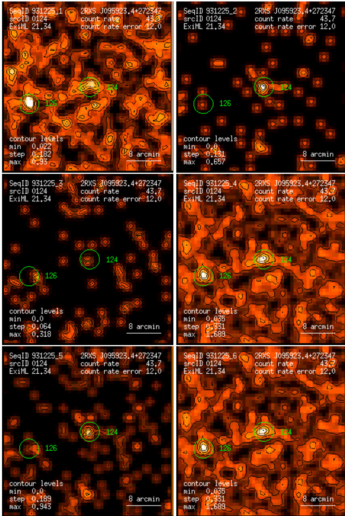
Figure 124: RASS 931225: detection 0124: band rate images, Gaussian filter: (1) PSPC channels 11 – 41, (2) 52 – 90, (3) 91 – 201, (4) 11 – 235, (5) 52 – 201, (6) 11 – 201. Broad band rates in counts/ks. Band rate contour levels in counts/ks/arcmin 2 .
