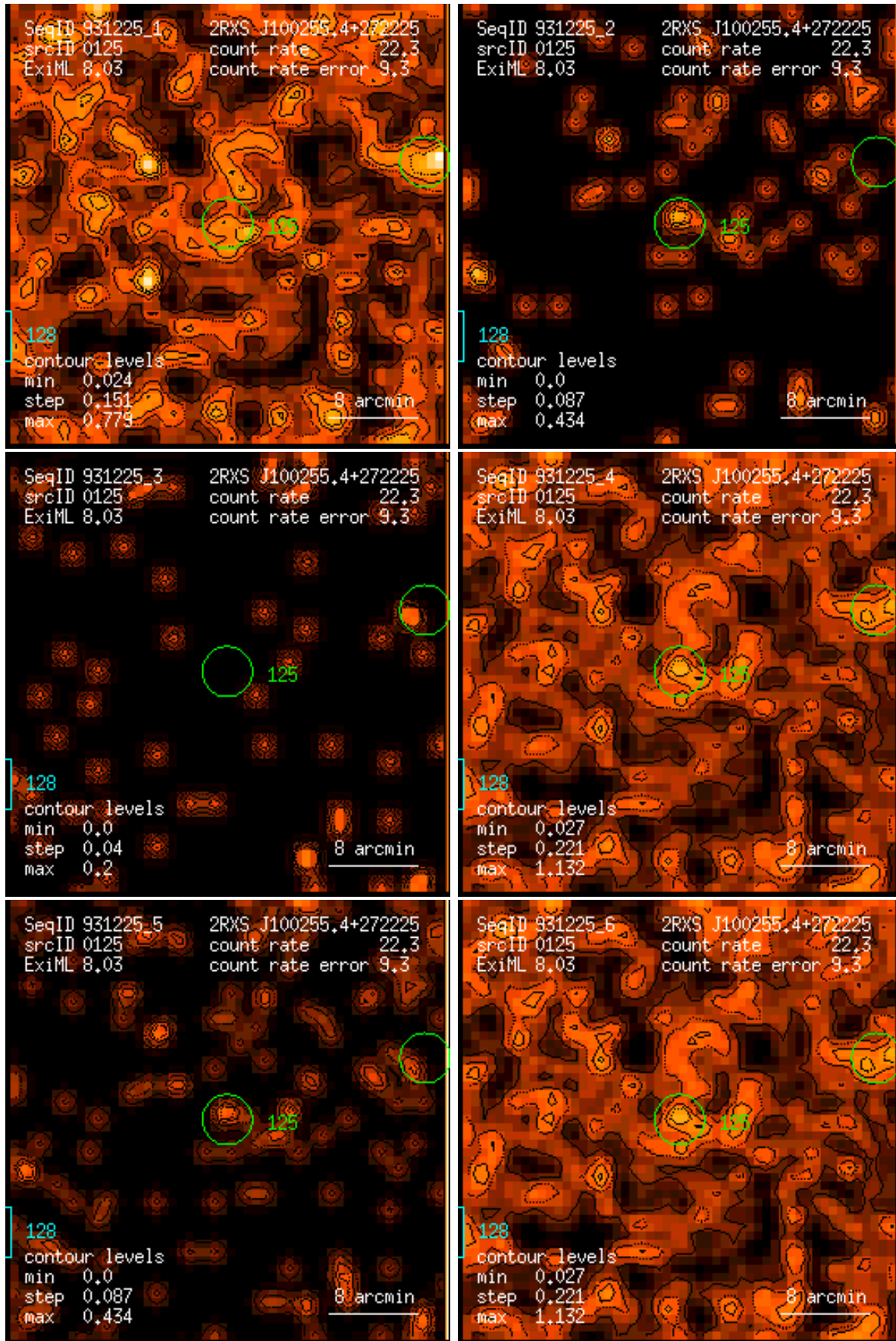
Figure 125: RASS 931225: detection 0125: band rate images, Gaussian filter: (1) PSPC channels 11 – 41, (2) 52 – 90, (3) 91 – 201, (4) 11 – 235, (5) 52 – 201, (6) 11 – 201. Broad band rates in counts/ks. Band rate contour levels in counts/ks/arcmin 2 .
