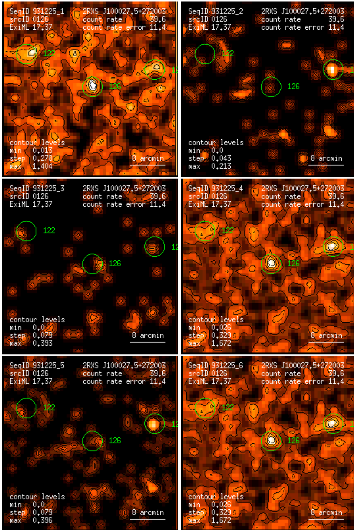
Figure 126: RASS 931225: detection 0126: band rate images, Gaussian filter: (1) PSPC channels 11 – 41, (2) 52 – 90, (3) 91 – 201, (4) 11 – 235, (5) 52 – 201, (6) 11 – 201. Broad band rates in counts/ks. Band rate contour levels in counts/ks/arcmin 2 .
