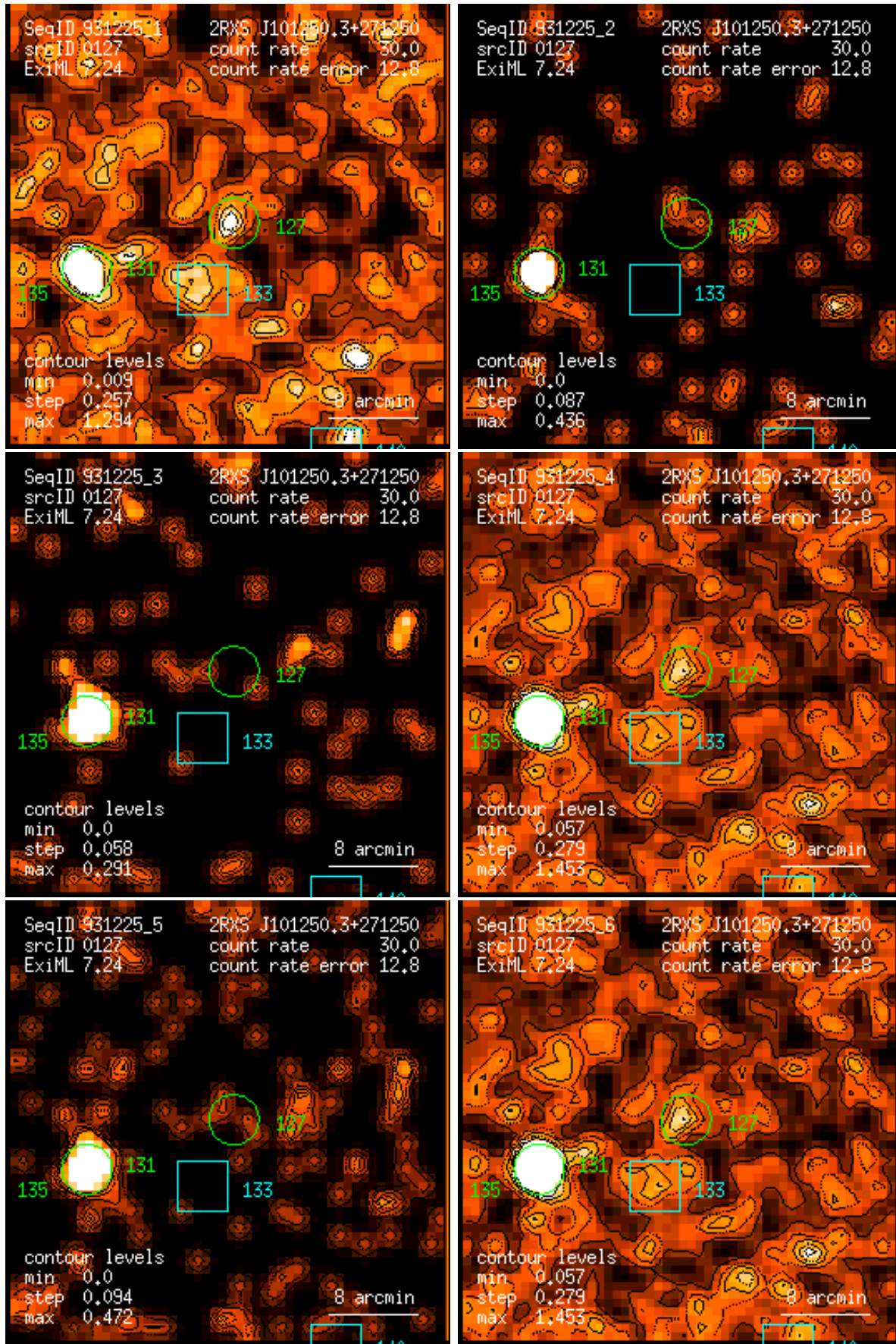
Figure 127: RASS 931225: detection 0127: band rate images, Gaussian filter: (1) PSPC channels 11 – 41, (2) 52 – 90, (3) 91 – 201, (4) 11 – 235, (5) 52 – 201, (6) 11 – 201. Broad band rates in counts/ks. Band rate contour levels in counts/ks/arcmin 2 .
