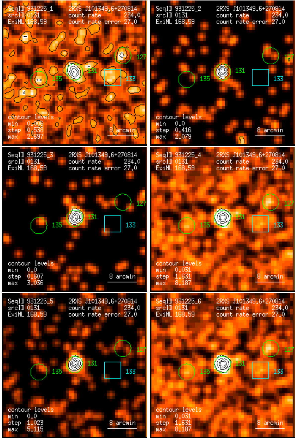
Figure 131: RASS 931225: detection 0131: band rate images, Gaussian filter: (1) PSPC channels 11 – 41, (2) 52 – 90, (3) 91 – 201, (4) 11 – 235, (5) 52 – 201, (6) 11 – 201. Broad band rates in counts/ks. Band rate contour levels in counts/ks/arcmin 2 .
