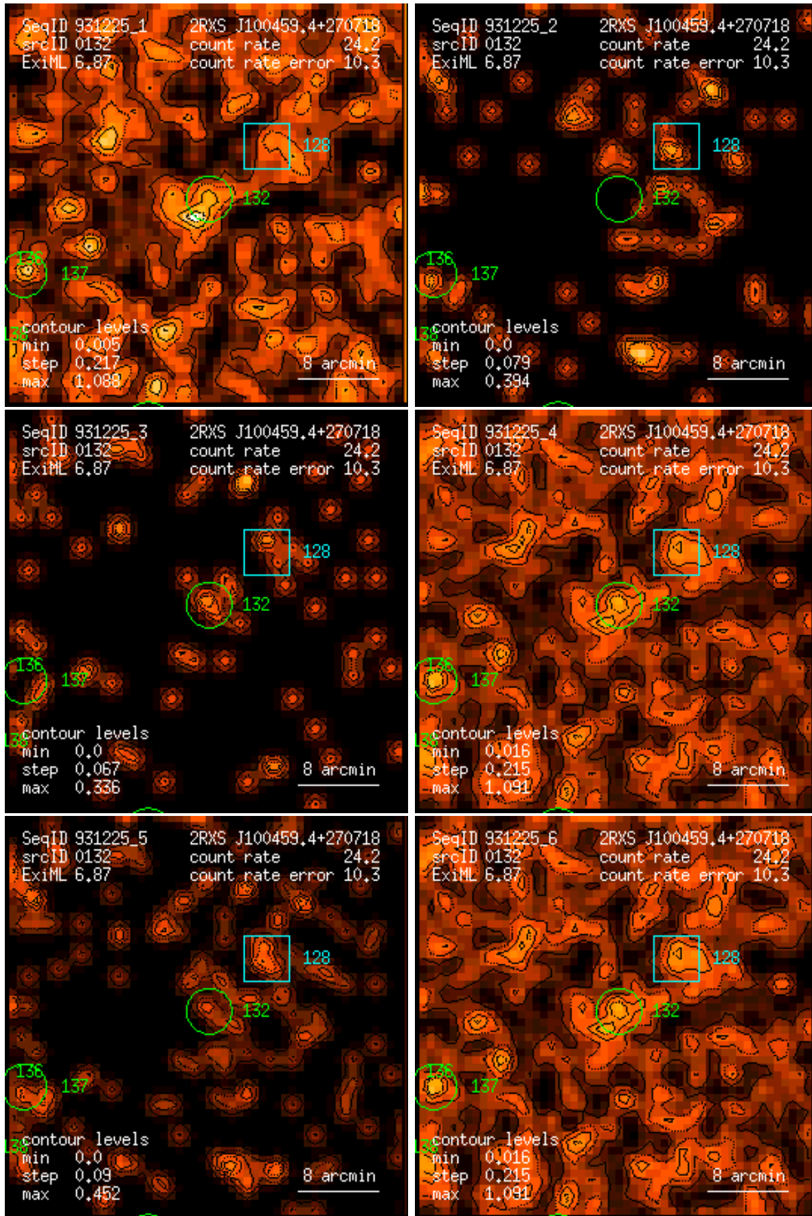
Figure 132: RASS 931225: detection 0132: band rate images, Gaussian filter: (1) PSPC channels 11 – 41, (2) 52 – 90, (3) 91 – 201, (4) 11 – 235, (5) 52 – 201, (6) 11 – 201. Broad band rates in counts/ks. Band rate contour levels in counts/ks/arcmin 2 .
