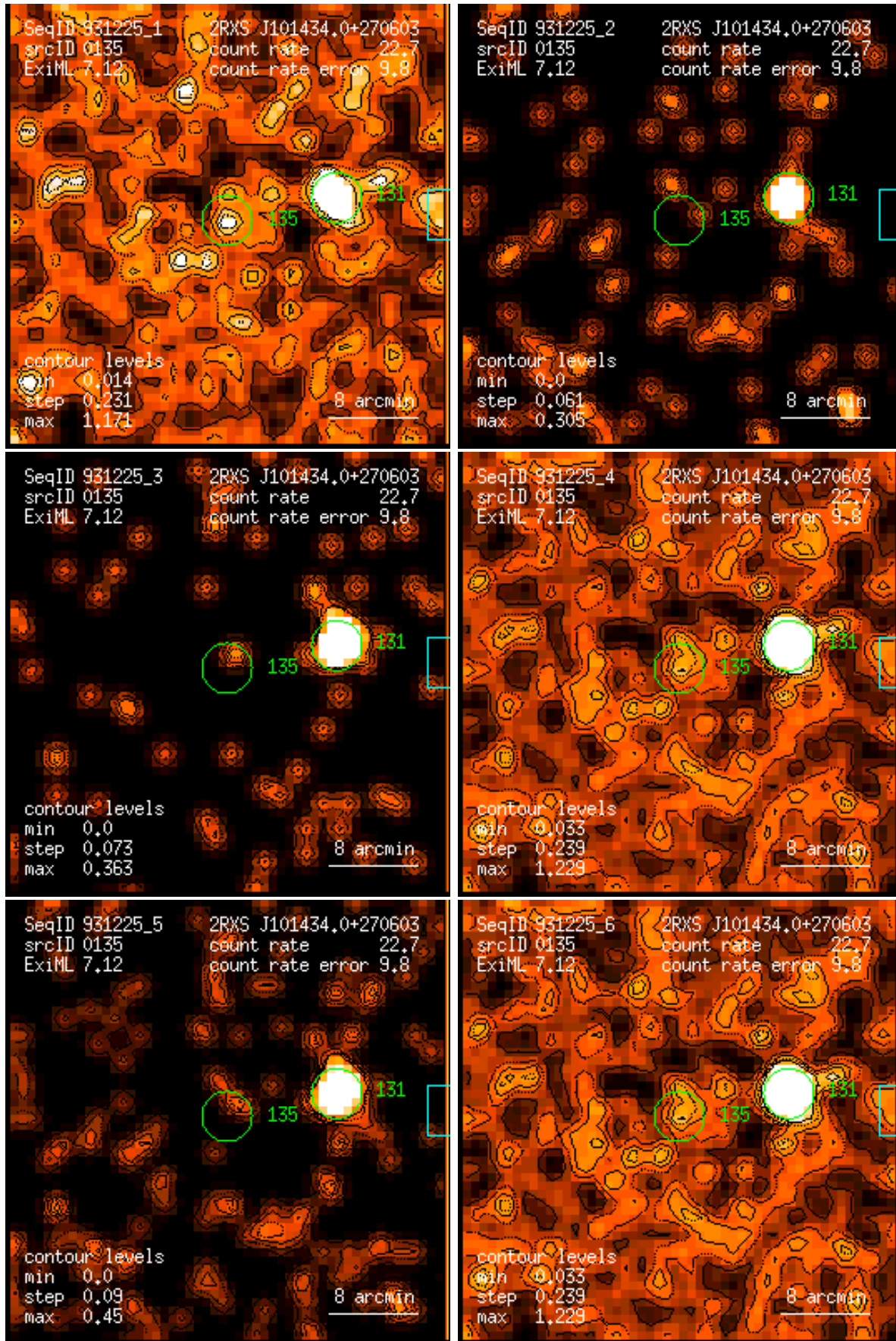
Figure 135: RASS 931225: detection 0135: band rate images, Gaussian filter: (1) PSPC channels 11 – 41, (2) 52 – 90, (3) 91 – 201, (4) 11 – 235, (5) 52 – 201, (6) 11 – 201. Broad band rates in counts/ks. Band rate contour levels in counts/ks/arcmin 2 .
