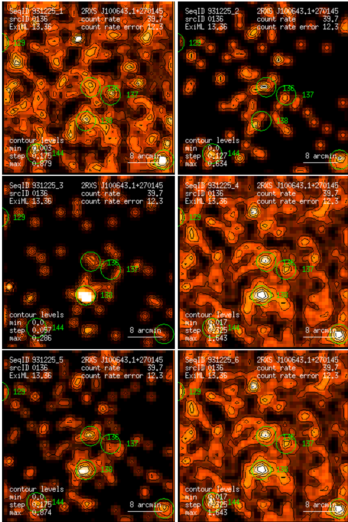
Figure 136: RASS 931225: detection 0136: band rate images, Gaussian filter: (1) PSPC channels 11 – 41, (2) 52 – 90, (3) 91 – 201, (4) 11 – 235, (5) 52 – 201, (6) 11 – 201. Broad band rates in counts/ks. Band rate contour levels in counts/ks/arcmin 2 .
