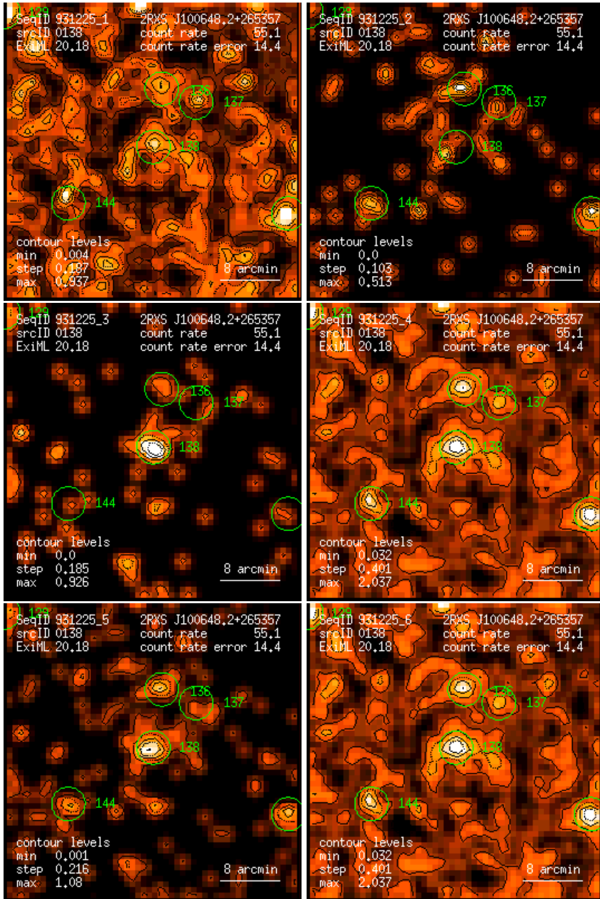
Figure 138: RASS 931225: detection 0138: band rate images, Gaussian filter: (1) PSPC channels 11 – 41, (2) 52 – 90, (3) 91 – 201, (4) 11 – 235, (5) 52 – 201, (6) 11 – 201. Broad band rates in counts/ks. Band rate contour levels in counts/ks/arcmin 2 .
