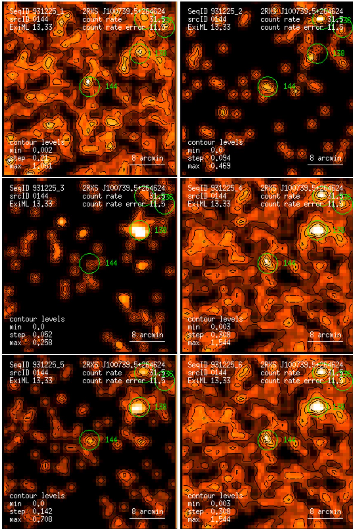
Figure 144: RASS 931225: detection 0144: band rate images, Gaussian filter: (1) PSPC channels 11 – 41, (2) 52 – 90, (3) 91 – 201, (4) 11 – 235, (5) 52 – 201, (6) 11 – 201. Broad band rates in counts/ks. Band rate contour levels in counts/ks/arcmin 2 .
