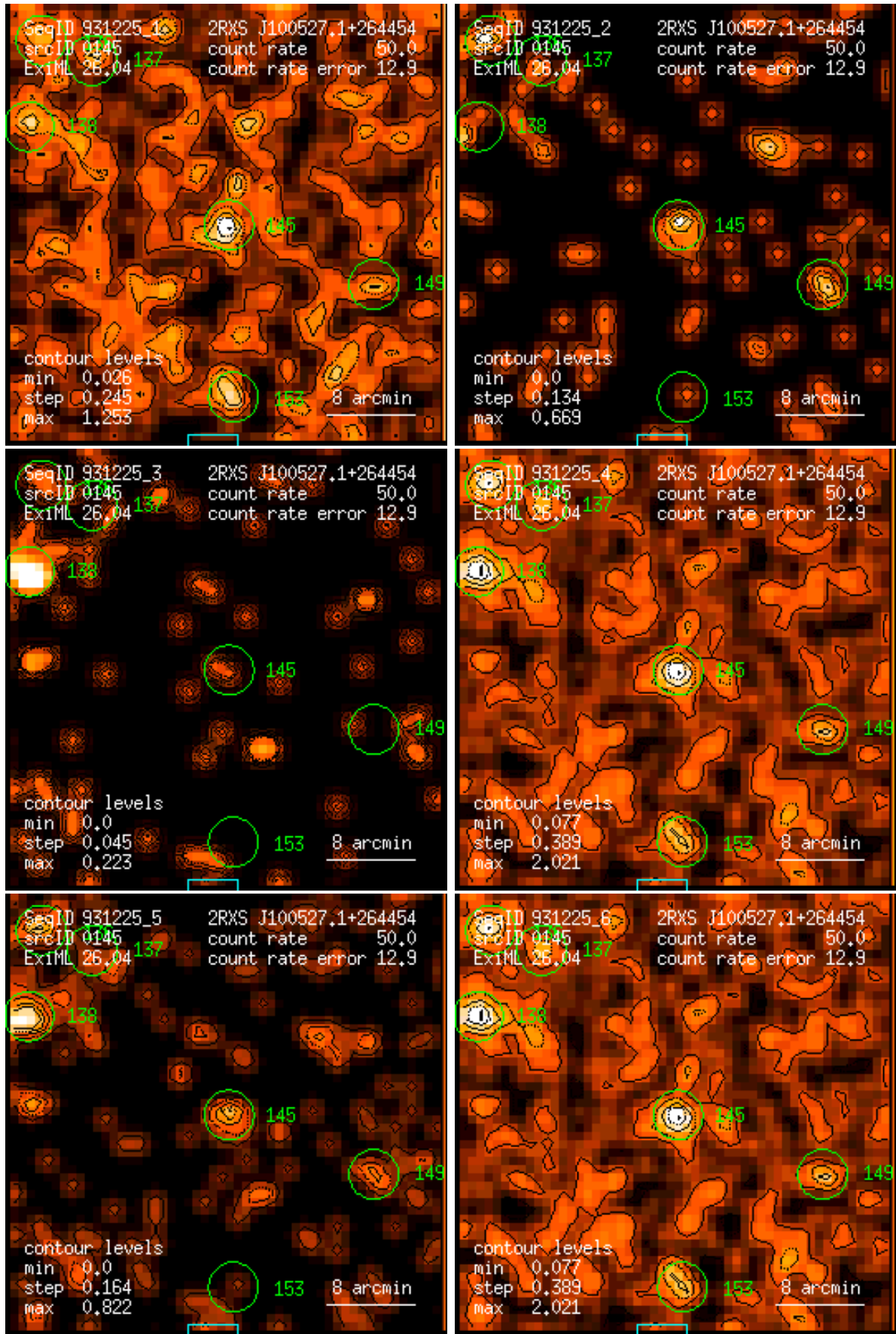
Figure 145: RASS 931225: detection 0145: band rate images, Gaussian filter: (1) PSPC channels 11 – 41, (2) 52 – 90, (3) 91 – 201, (4) 11 – 235, (5) 52 – 201, (6) 11 – 201. Broad band rates in counts/ks. Band rate contour levels in counts/ks/arcmin 2 .
