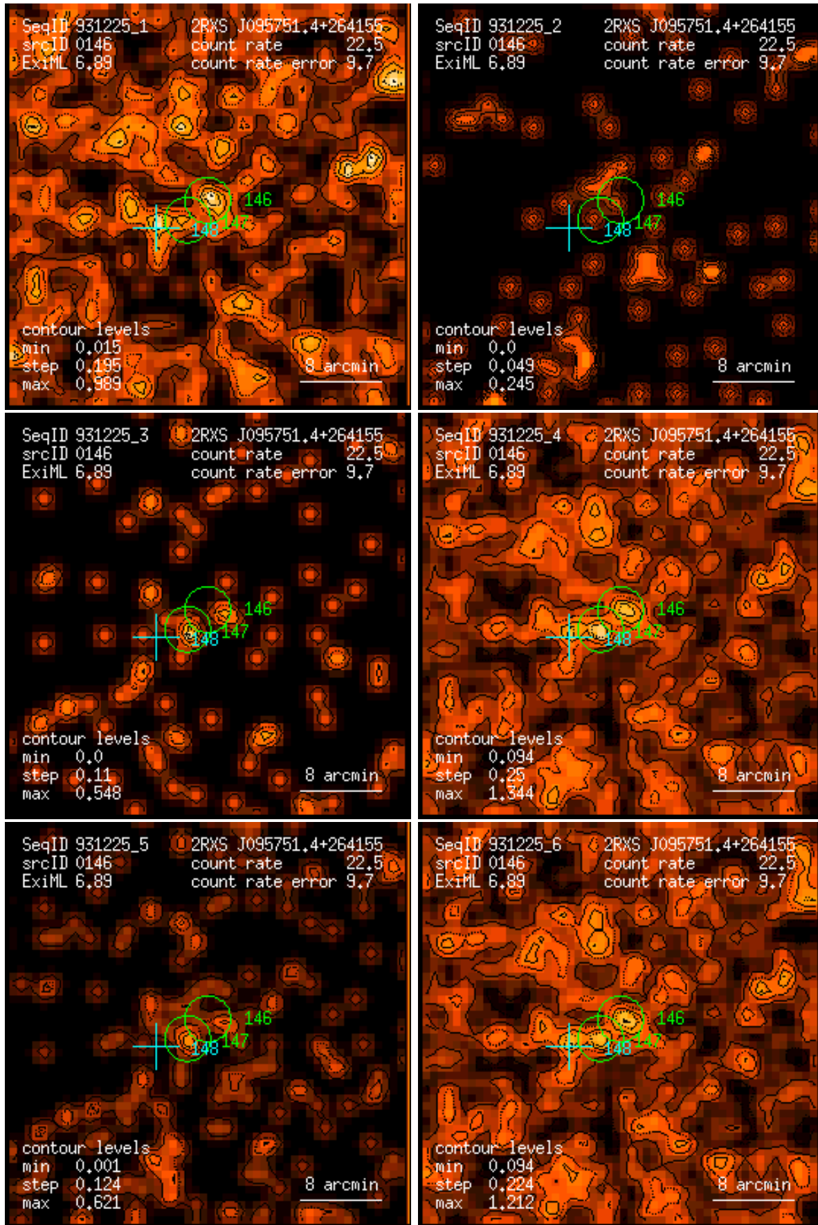
Figure 146: RASS 931225: detection 0146: band rate images, Gaussian filter: (1) PSPC channels 11 – 41, (2) 52 – 90, (3) 91 – 201, (4) 11 – 235, (5) 52 – 201, (6) 11 – 201. Broad band rates in counts/ks. Band rate contour levels in counts/ks/arcmin 2 .
