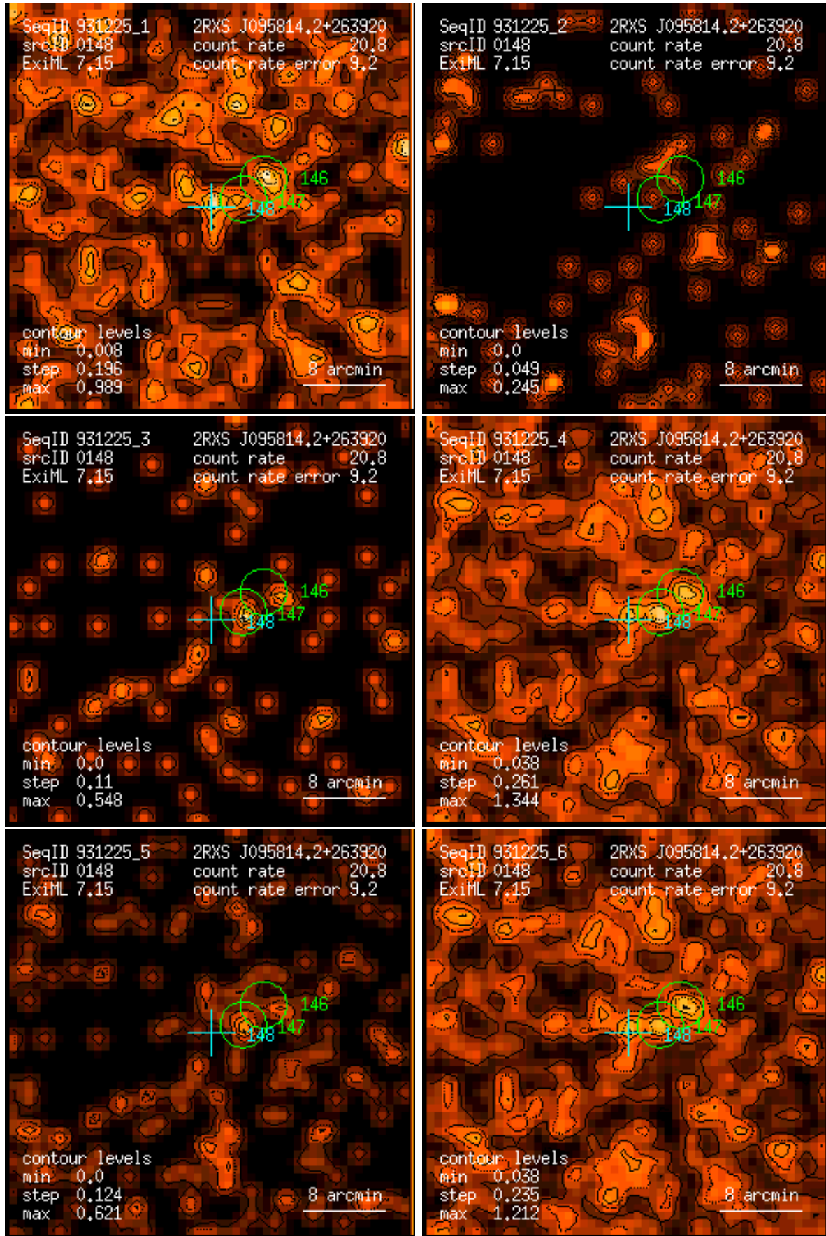
Figure 148: RASS 931225: detection 0148: band rate images, Gaussian filter: (1) PSPC channels 11 – 41, (2) 52 – 90, (3) 91 – 201, (4) 11 – 235, (5) 52 – 201, (6) 11 – 201. Broad band rates in counts/ks. Band rate contour levels in counts/ks/arcmin 2 .
