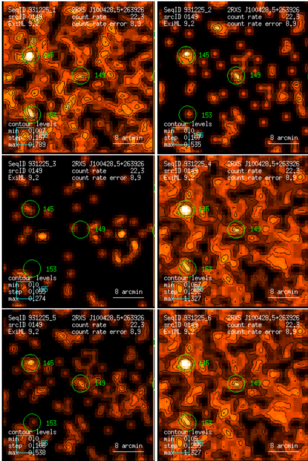
Figure 149: RASS 931225: detection 0149: band rate images, Gaussian filter: (1) PSPC channels 11 – 41, (2) 52 – 90, (3) 91 – 201, (4) 11 – 235, (5) 52 – 201, (6) 11 – 201. Broad band rates in counts/ks. Band rate contour levels in counts/ks/arcmin 2 .
