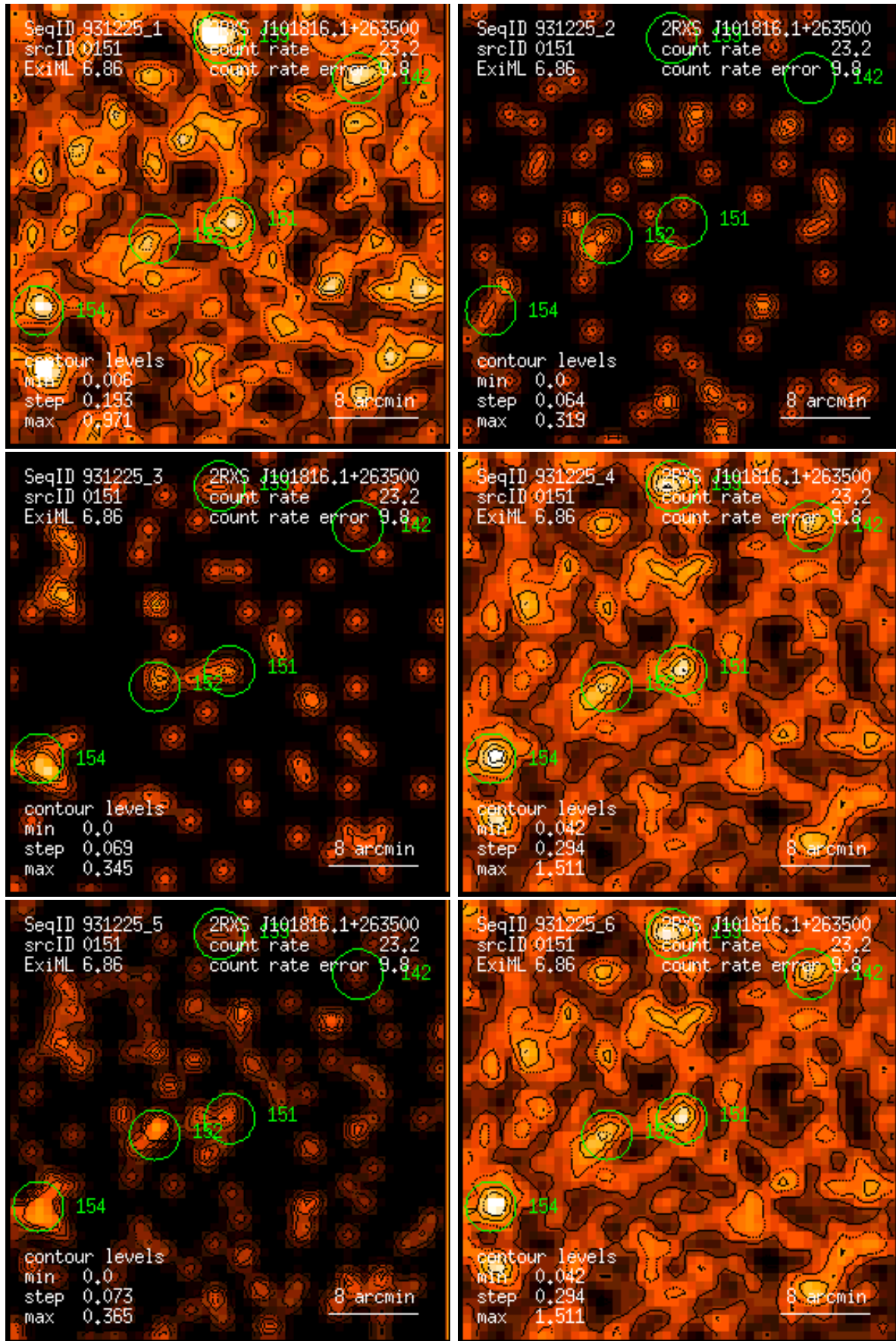
Figure 151: RASS 931225: detection 0151: band rate images, Gaussian filter: (1) PSPC channels 11 – 41, (2) 52 – 90, (3) 91 – 201, (4) 11 – 235, (5) 52 – 201, (6) 11 – 201. Broad band rates in counts/ks. Band rate contour levels in counts/ks/arcmin 2 .
