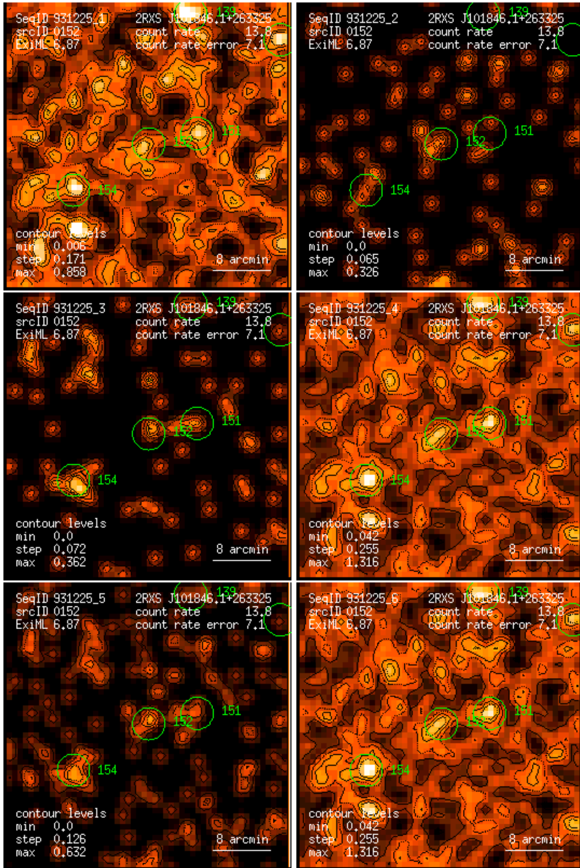
Figure 152: RASS 931225: detection 0152: band rate images, Gaussian filter: (1) PSPC channels 11 – 41, (2) 52 – 90, (3) 91 – 201, (4) 11 – 235, (5) 52 – 201, (6) 11 – 201. Broad band rates in counts/ks. Band rate contour levels in counts/ks/arcmin 2 .
