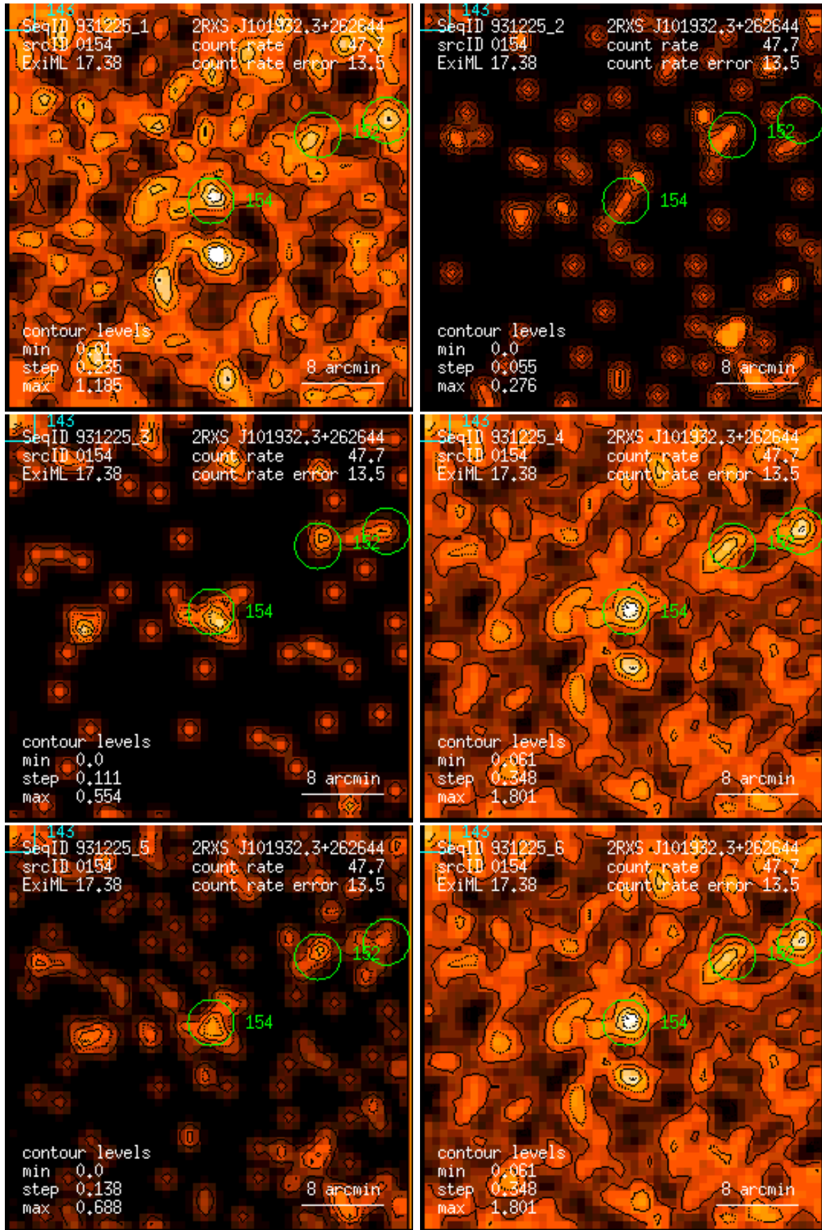
Figure 154: RASS 931225: detection 0154: band rate images, Gaussian filter: (1) PSPC channels 11 – 41, (2) 52 – 90, (3) 91 – 201, (4) 11 – 235, (5) 52 – 201, (6) 11 – 201. Broad band rates in counts/ks. Band rate contour levels in counts/ks/arcmin 2 .
