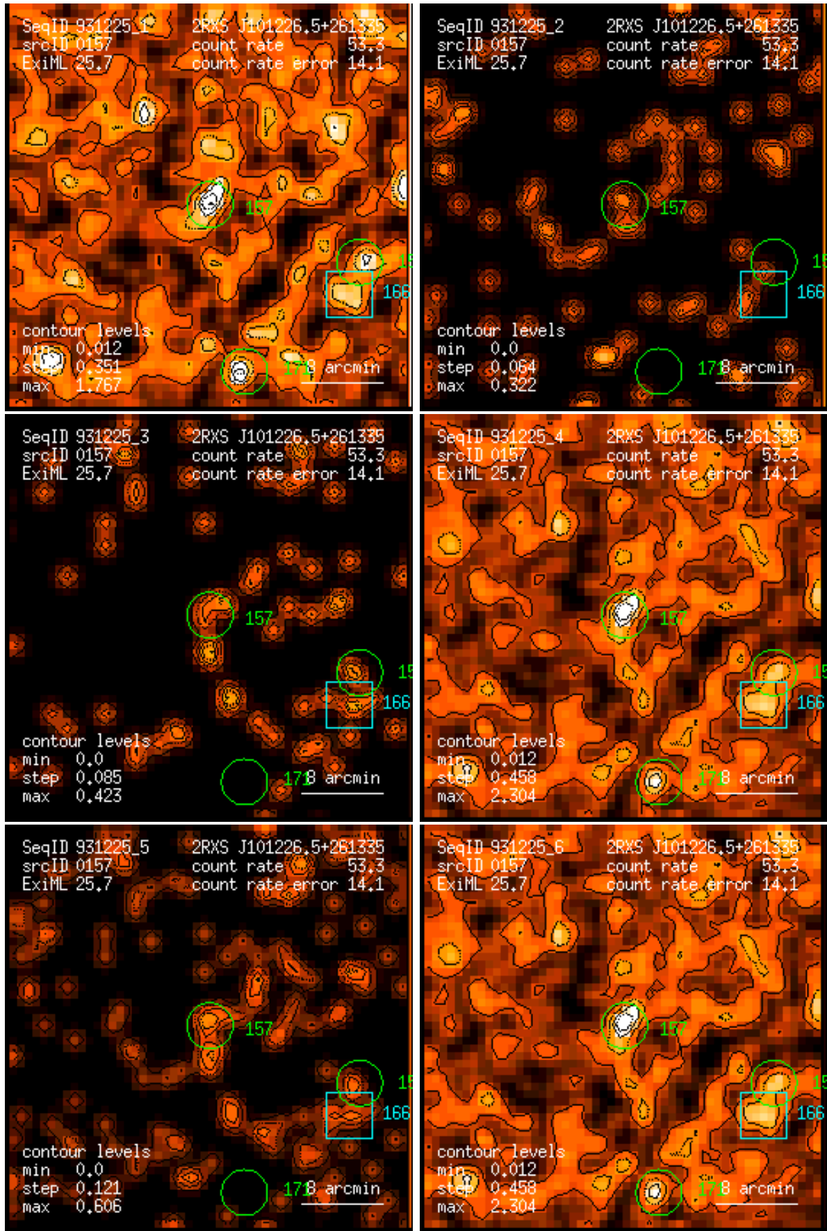
Figure 157: RASS 931225: detection 0157: band rate images, Gaussian filter: (1) PSPC channels 11 – 41, (2) 52 – 90, (3) 91 – 201, (4) 11 – 235, (5) 52 – 201, (6) 11 – 201. Broad band rates in counts/ks. Band rate contour levels in counts/ks/arcmin 2 .
