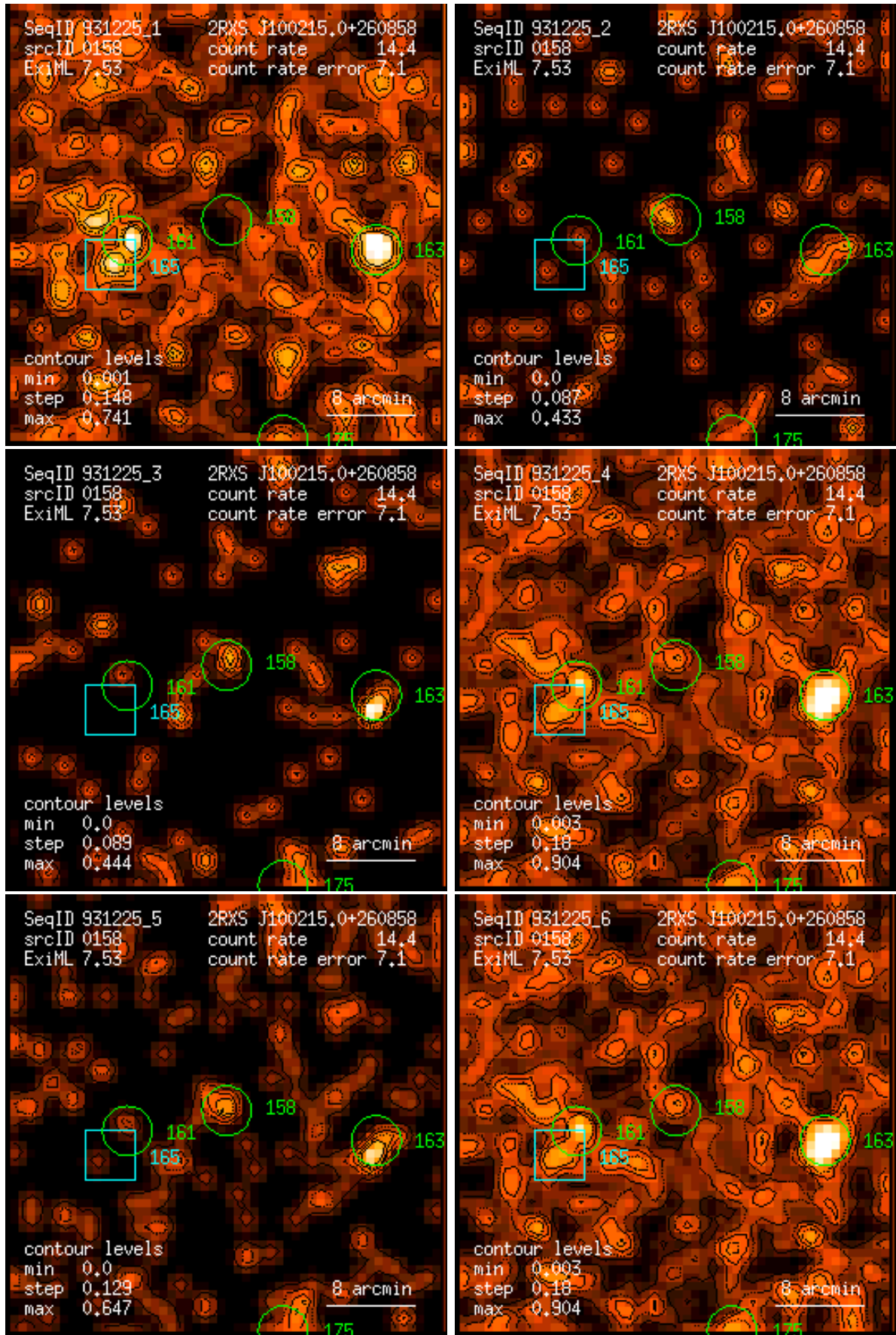
Figure 158: RASS 931225: detection 0158: band rate images, Gaussian filter: (1) PSPC channels 11 – 41, (2) 52 – 90, (3) 91 – 201, (4) 11 – 235, (5) 52 – 201, (6) 11 – 201. Broad band rates in counts/ks. Band rate contour levels in counts/ks/arcmin 2 .
