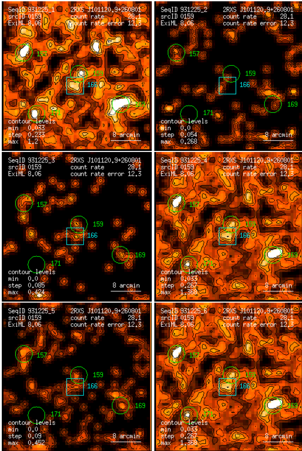
Figure 159: RASS 931225: detection 0159: band rate images, Gaussian filter: (1) PSPC channels 11 – 41, (2) 52 – 90, (3) 91 – 201, (4) 11 – 235, (5) 52 – 201, (6) 11 – 201. Broad band rates in counts/ks. Band rate contour levels in counts/ks/arcmin 2 .
