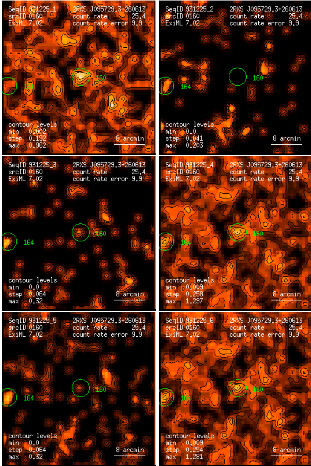
Figure 160: RASS 931225: detection 0160: band rate images, Gaussian filter: (1) PSPC channels 11 – 41, (2) 52 – 90, (3) 91 – 201, (4) 11 – 235, (5) 52 – 201, (6) 11 – 201. Broad band rates in counts/ks. Band rate contour levels in counts/ks/arcmin 2 .
