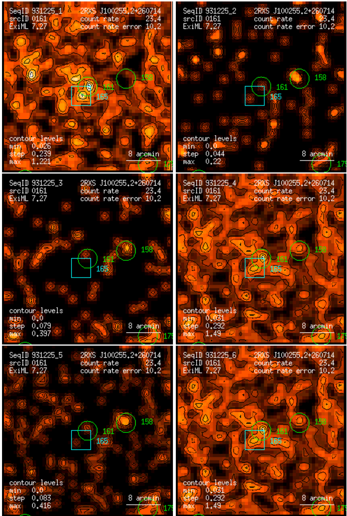
Figure 161: RASS 931225: detection 0161: band rate images, Gaussian filter: (1) PSPC channels 11 – 41, (2) 52 – 90, (3) 91 – 201, (4) 11 – 235, (5) 52 – 201, (6) 11 – 201. Broad band rates in counts/ks. Band rate contour levels in counts/ks/arcmin 2 .
