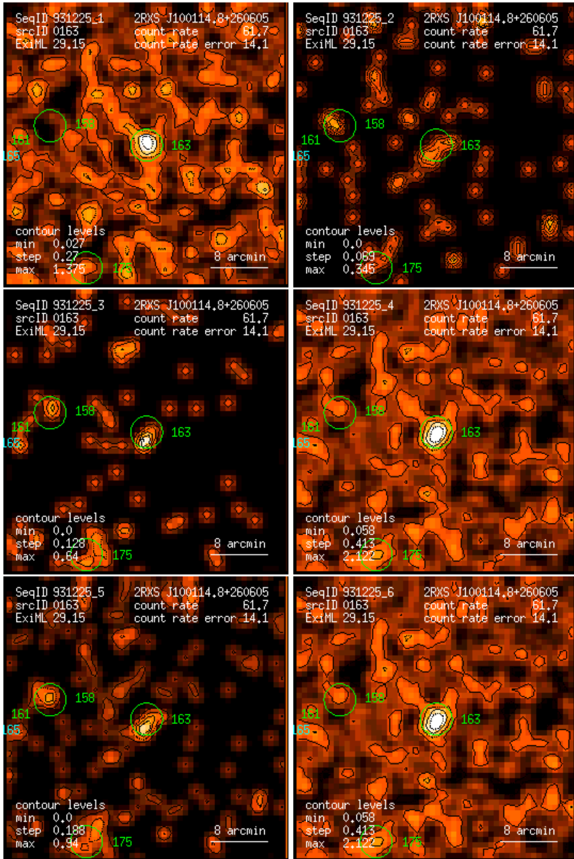
Figure 163: RASS 931225: detection 0163: band rate images, Gaussian filter: (1) PSPC channels 11 – 41, (2) 52 – 90, (3) 91 – 201, (4) 11 – 235, (5) 52 – 201, (6) 11 – 201. Broad band rates in counts/ks. Band rate contour levels in counts/ks/arcmin 2 .
