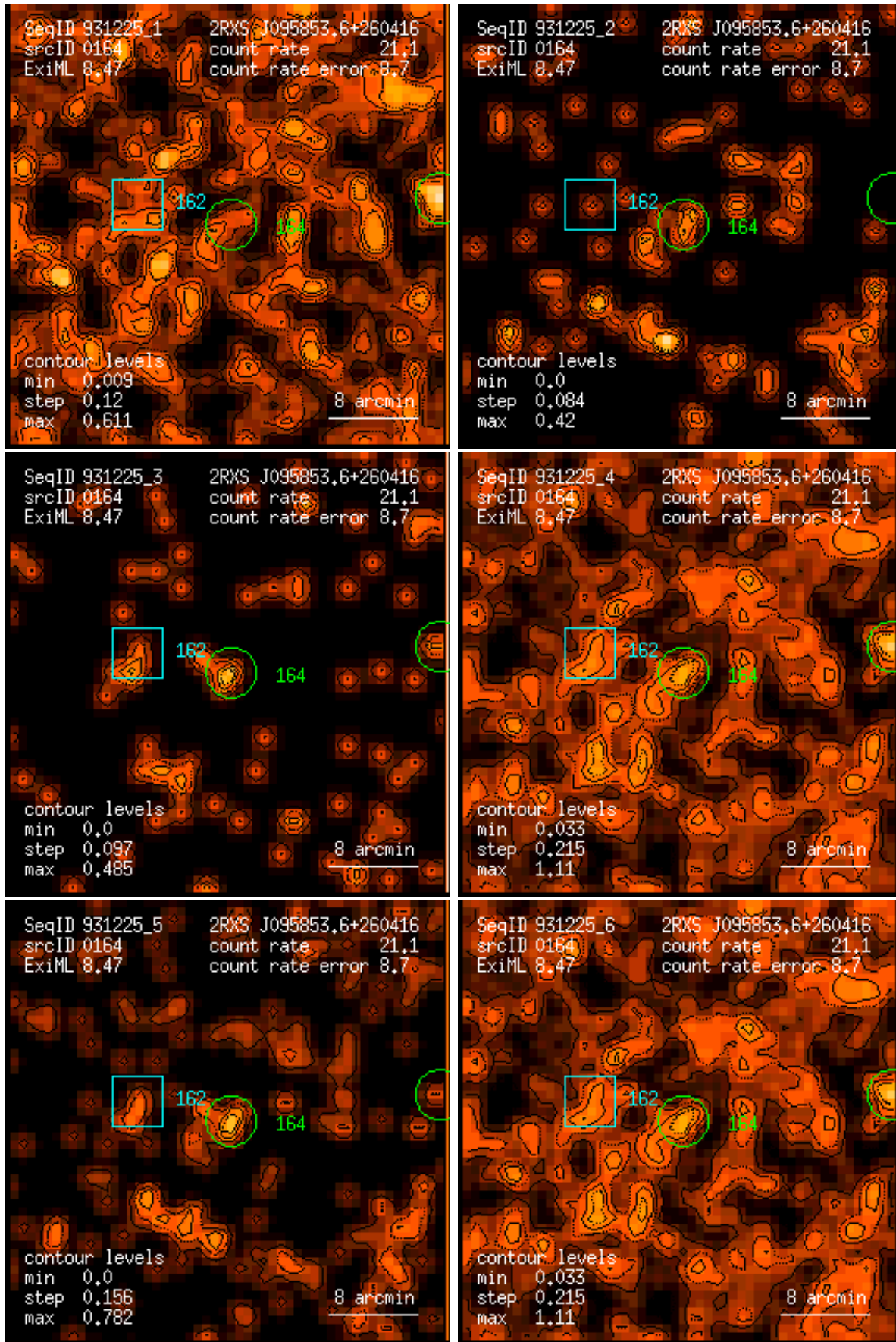
Figure 164: RASS 931225: detection 0164: band rate images, Gaussian filter: (1) PSPC channels 11 – 41, (2) 52 – 90, (3) 91 – 201, (4) 11 – 235, (5) 52 – 201, (6) 11 – 201. Broad band rates in counts/ks. Band rate contour levels in counts/ks/arcmin 2 .
