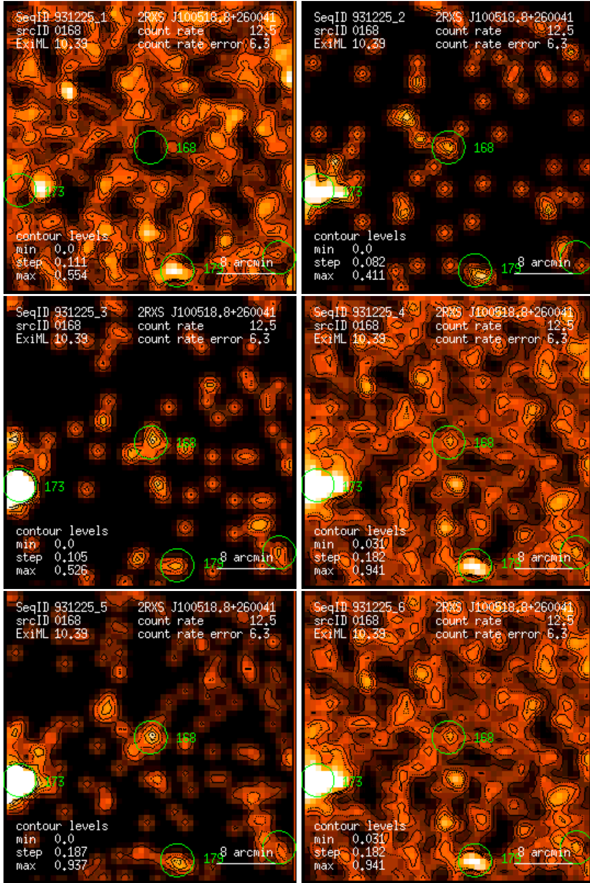
Figure 168: RASS 931225: detection 0168: band rate images, Gaussian filter: (1) PSPC channels 11 – 41, (2) 52 – 90, (3) 91 – 201, (4) 11 – 235, (5) 52 – 201, (6) 11 – 201. Broad band rates in counts/ks. Band rate contour levels in counts/ks/arcmin 2 .
