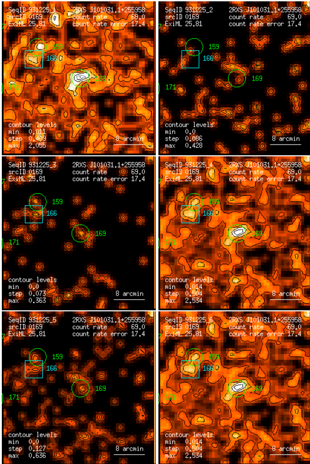
Figure 169: RASS 931225: detection 0169: band rate images, Gaussian filter: (1) PSPC channels 11 – 41, (2) 52 – 90, (3) 91 – 201, (4) 11 – 235, (5) 52 – 201, (6) 11 – 201. Broad band rates in counts/ks. Band rate contour levels in counts/ks/arcmin 2 .
