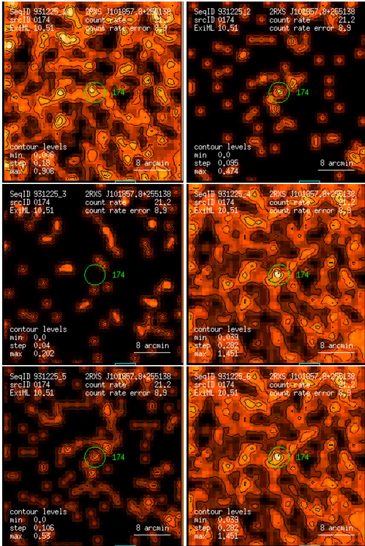
Figure 174: RASS 931225: detection 0174: band rate images, Gaussian filter: (1) PSPC channels 11 – 41, (2) 52 – 90, (3) 91 – 201, (4) 11 – 235, (5) 52 – 201, (6) 11 – 201. Broad band rates in counts/ks. Band rate contour levels in counts/ks/arcmin 2 .
