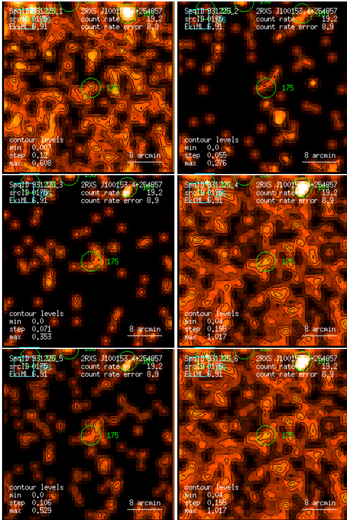
Figure 175: RASS 931225: detection 0175: band rate images, Gaussian filter: (1) PSPC channels 11 – 41, (2) 52 – 90, (3) 91 – 201, (4) 11 – 235, (5) 52 – 201, (6) 11 – 201. Broad band rates in counts/ks. Band rate contour levels in counts/ks/arcmin 2 .
