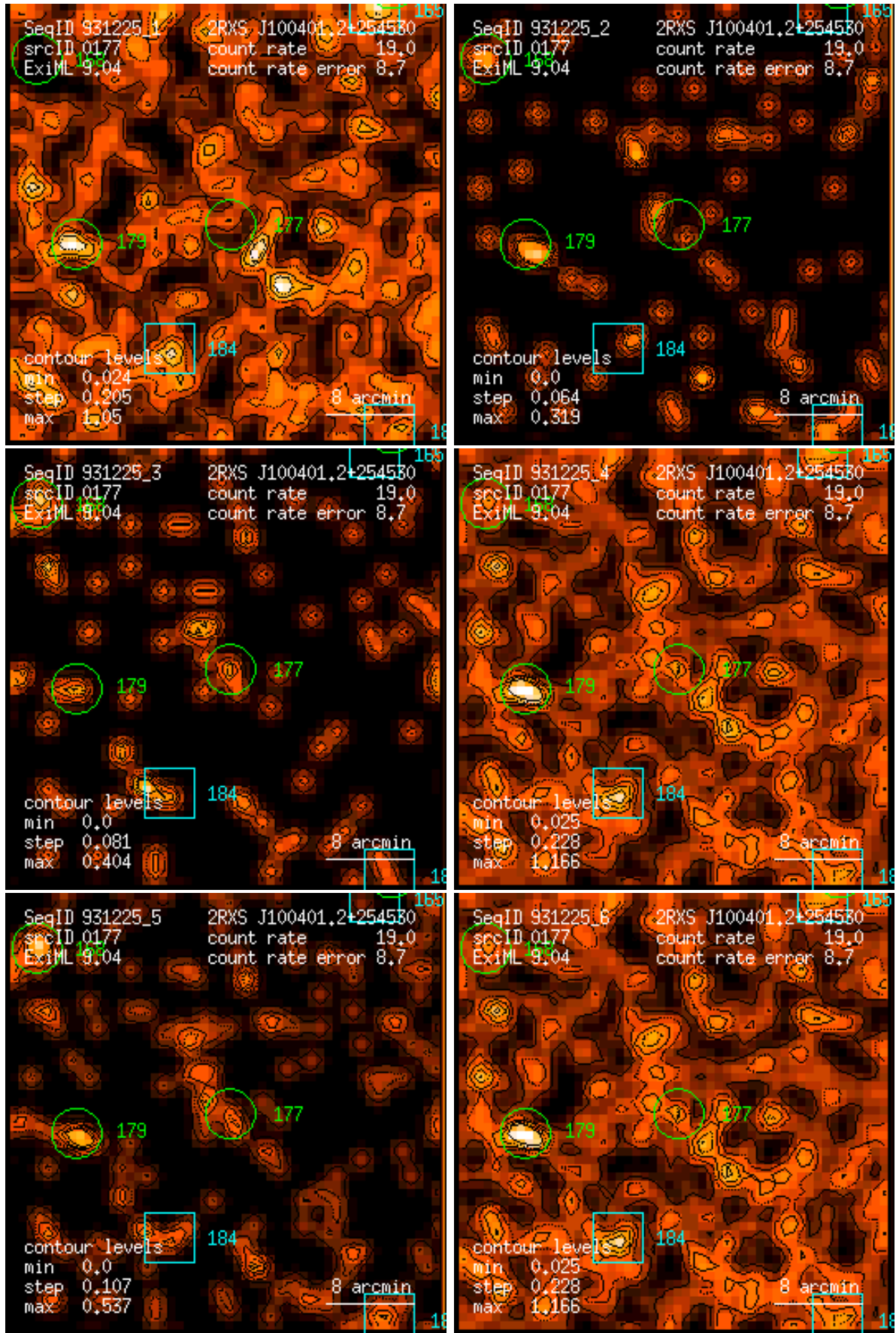
Figure 177: RASS 931225: detection 0177: band rate images, Gaussian filter: (1) PSPC channels 11 – 41, (2) 52 – 90, (3) 91 – 201, (4) 11 – 235, (5) 52 – 201, (6) 11 – 201. Broad band rates in counts/ks. Band rate contour levels in counts/ks/arcmin 2 .
