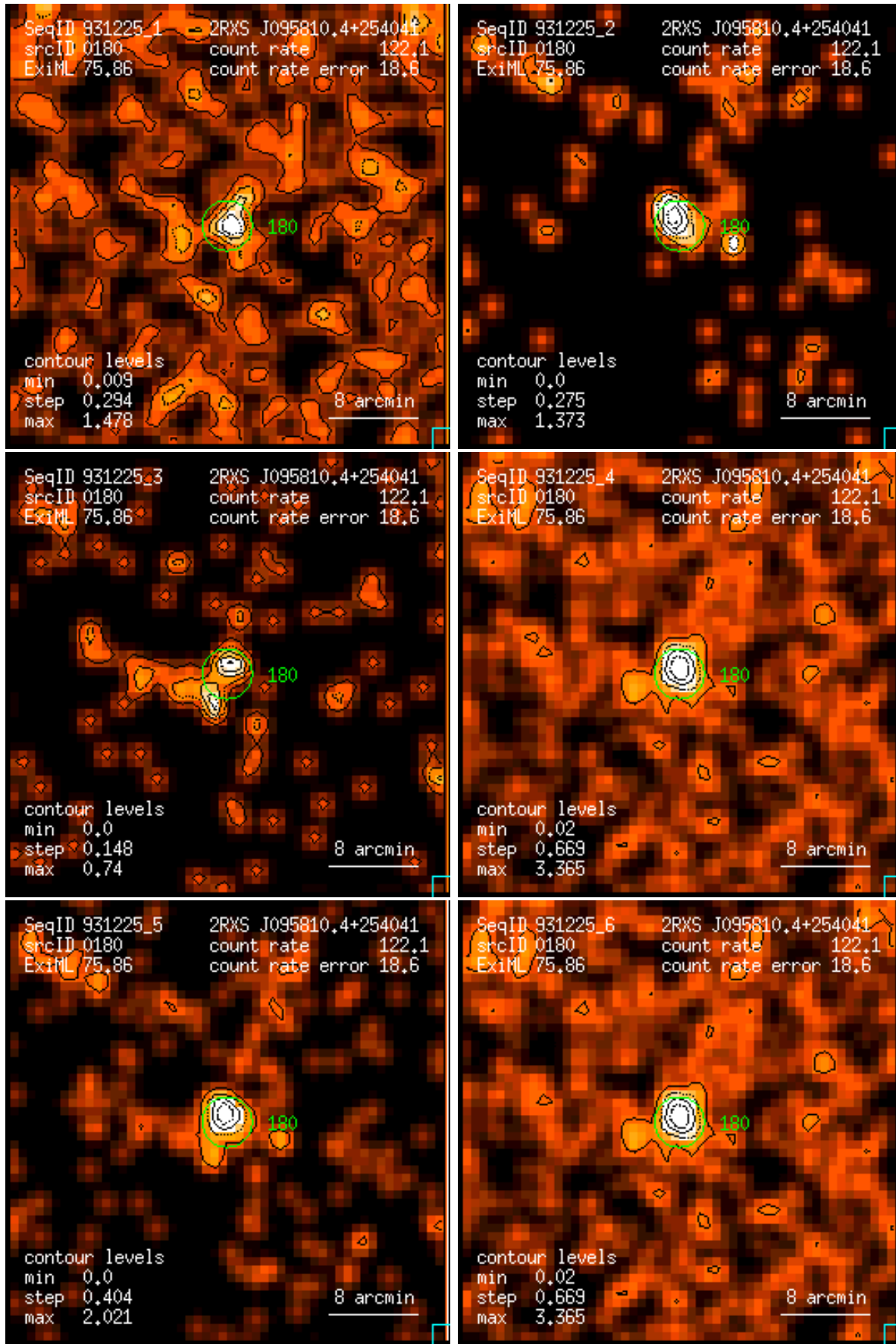
Figure 180: RASS 931225: detection 0180: band rate images, Gaussian filter: (1) PSPC channels 11 – 41, (2) 52 – 90, (3) 91 – 201, (4) 11 – 235, (5) 52 – 201, (6) 11 – 201. Broad band rates in counts/ks. Band rate contour levels in counts/ks/arcmin 2 .
