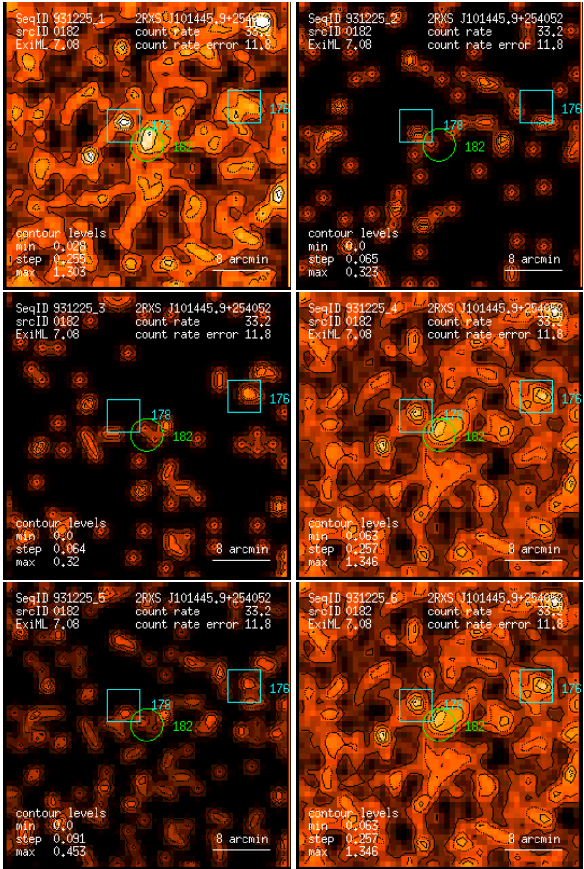
Figure 182: RASS 931225: detection 0182: band rate images, Gaussian filter: (1) PSPC channels 11 – 41, (2) 52 – 90, (3) 91 – 201, (4) 11 – 235, (5) 52 – 201, (6) 11 – 201. Broad band rates in counts/ks. Band rate contour levels in counts/ks/arcmin 2 .
