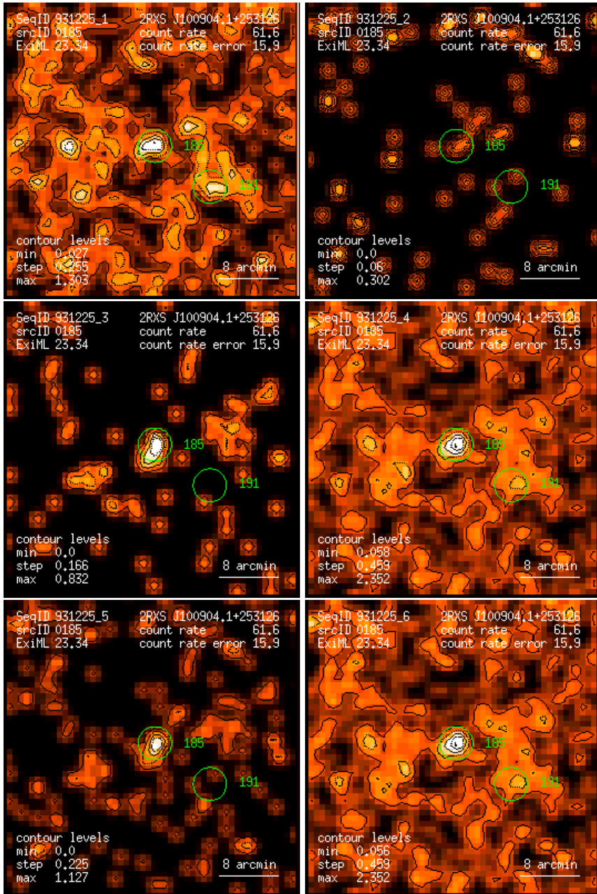
Figure 185: RASS 931225: detection 0185: band rate images, Gaussian filter: (1) PSPC channels 11 – 41, (2) 52 – 90, (3) 91 – 201, (4) 11 – 235, (5) 52 – 201, (6) 11 – 201. Broad band rates in counts/ks. Band rate contour levels in counts/ks/arcmin 2 .
