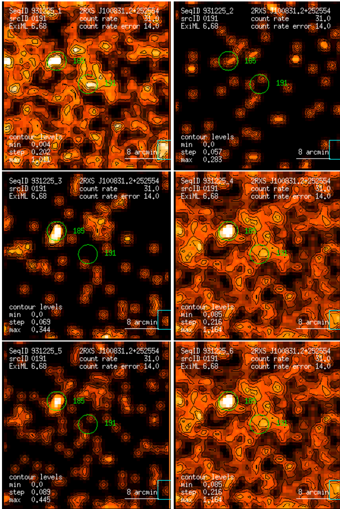
Figure 191: RASS 931225: detection 0191: band rate images, Gaussian filter: (1) PSPC channels 11 – 41, (2) 52 – 90, (3) 91 – 201, (4) 11 – 235, (5) 52 – 201, (6) 11 – 201. Broad band rates in counts/ks. Band rate contour levels in counts/ks/arcmin 2 .
