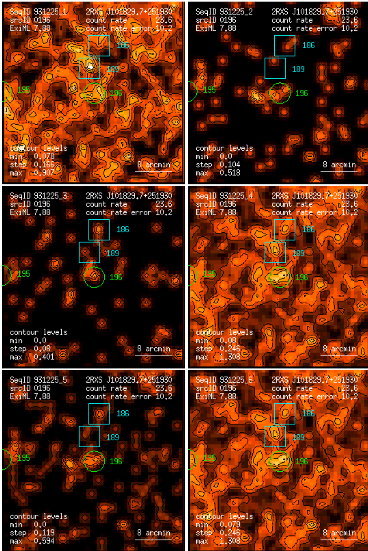
Figure 196: RASS 931225: detection 0196: band rate images, Gaussian filter: (1) PSPC channels 11 – 41, (2) 52 – 90, (3) 91 – 201, (4) 11 – 235, (5) 52 – 201, (6) 11 – 201. Broad band rates in counts/ks. Band rate contour levels in counts/ks/arcmin 2 .
