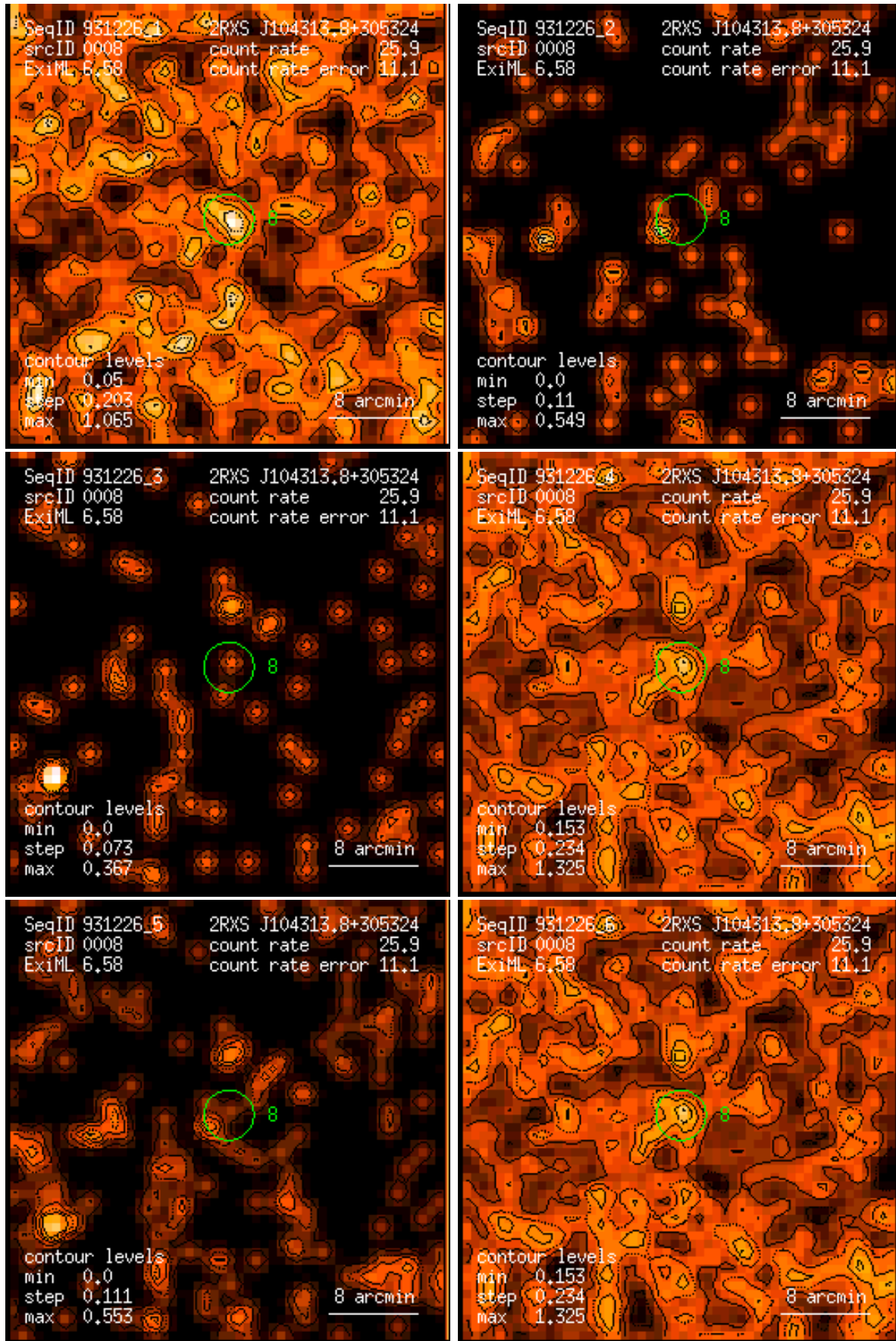
Figure 8: RASS 931226: detection 0008: band rate images, Gaussian filter: (1) PSPC channels 11 – 41, (2) 52 – 90, (3) 91 – 201, (4) 11 – 235, (5) 52 – 201, (6) 11 – 201. Broad band rates in counts/ks. Band rate contour levels in counts/ks/arcmin 2 .
