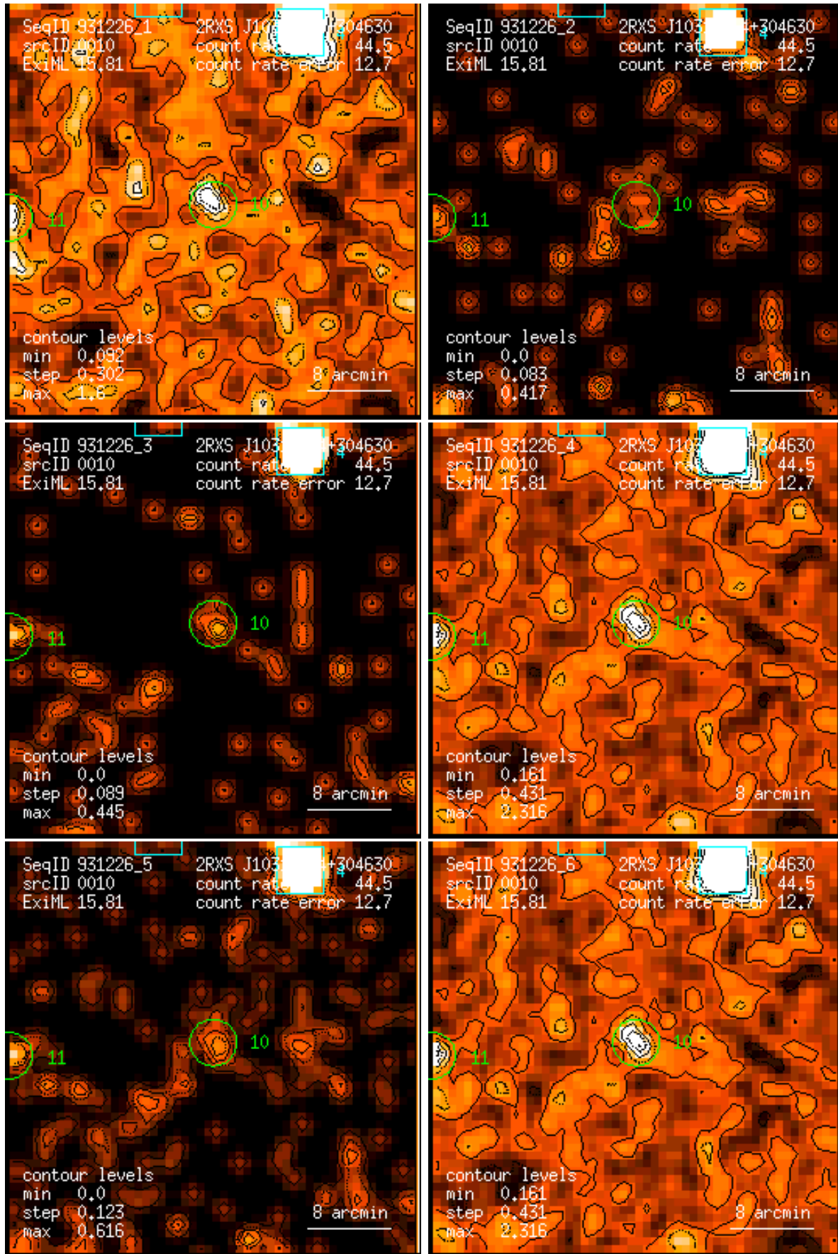
Figure 10: RASS 931226: detection 0010: band rate images, Gaussian filter: (1) PSPC channels 11 – 41, (2) 52 – 90, (3) 91 – 201, (4) 11 – 235, (5) 52 – 201, (6) 11 – 201. Broad band rates in counts/ks. Band rate contour levels in counts/ks/arcmin 2 .
