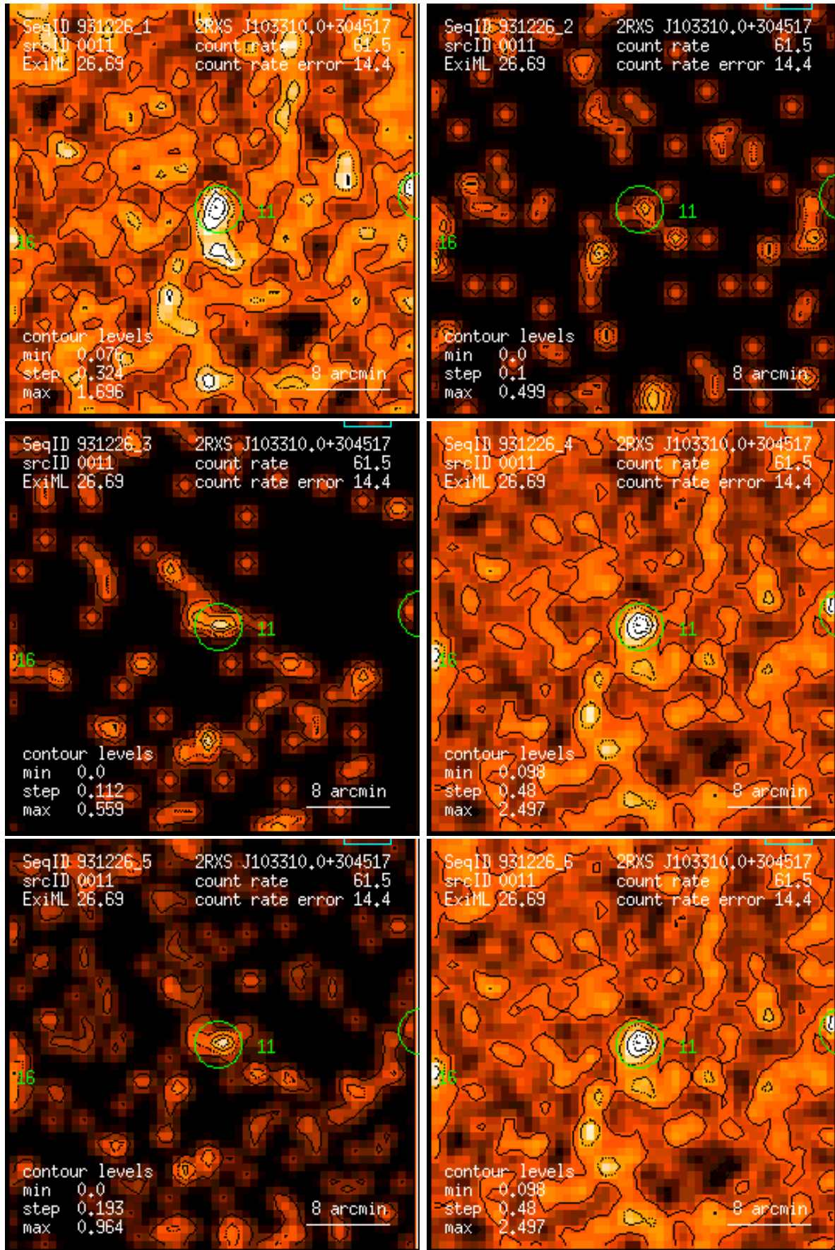
Figure 11: RASS 931226: detection 0011: band rate images, Gaussian filter: (1) PSPC channels 11 – 41, (2) 52 – 90, (3) 91 – 201, (4) 11 – 235, (5) 52 – 201, (6) 11 – 201. Broad band rates in counts/ks. Band rate contour levels in counts/ks/arcmin 2 .
