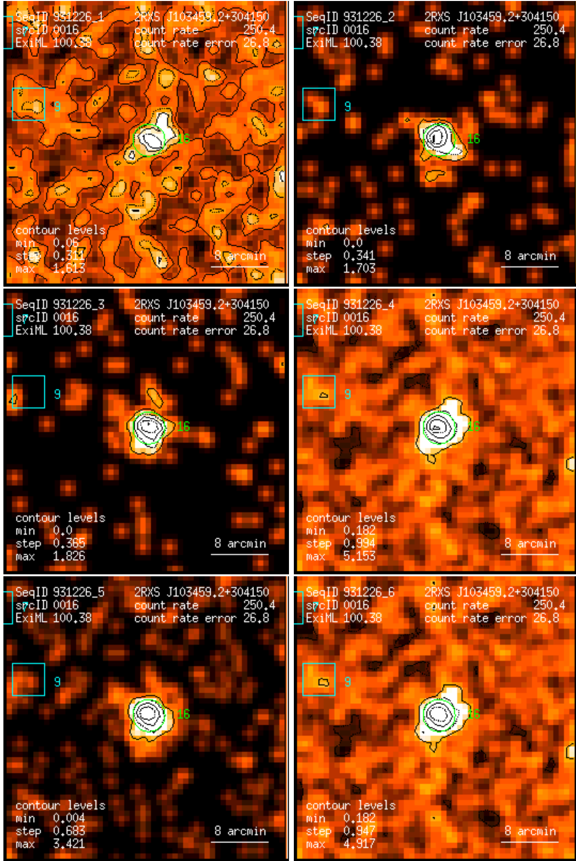
Figure 16: RASS 931226: detection 0016: band rate images, Gaussian filter: (1) PSPC channels 11 – 41, (2) 52 – 90, (3) 91 – 201, (4) 11 – 235, (5) 52 – 201, (6) 11 – 201. Broad band rates in counts/ks. Band rate contour levels in counts/ks/arcmin 2 .
